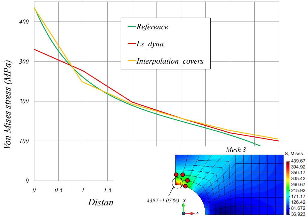
Figure 3.25: von-Mises st
