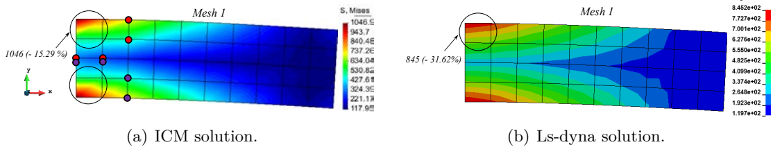
Figure 3.33: Von-Mises stress contour maps of clamped beam in Mesh 1.
