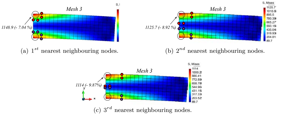
Figure 3.39: Von-Mises stress distribution: influence of surrounding nodes.
