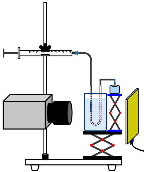
Fig. 6.1 Experimental setup used for investigating influence of temperature on polymerization of glue-Lipiodol mixtures. A U-shaped capillary tube is immersed in a water bath.
