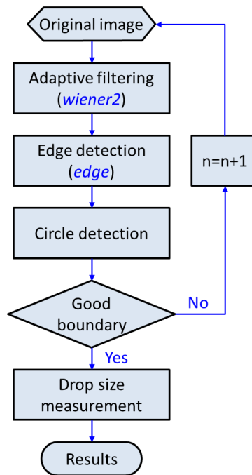
Fig. 2.11 Flow diagram of the image processing for drop size measurements.
