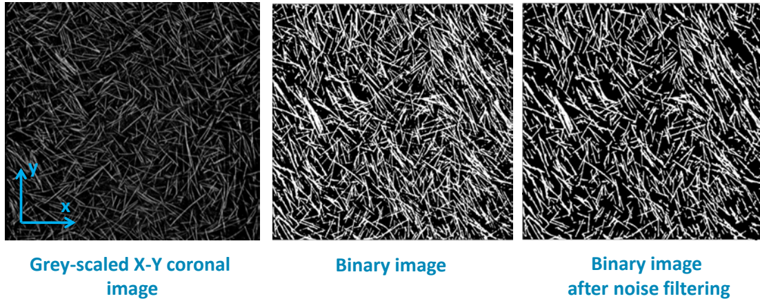
Figure 4.20: Treatment of 2D grey-scaled images obtained from \mu -CT scan of a PP-30GF specimen
