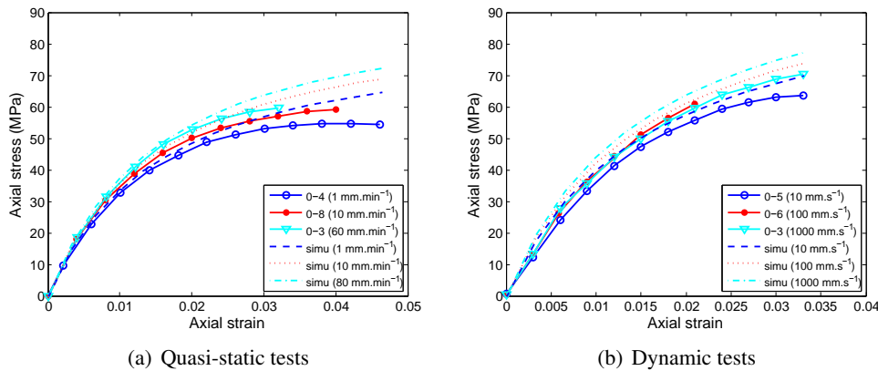
Figure 4.47: Comparison of experimental and numerical data for tests of 45° specimens of PP-40GF
