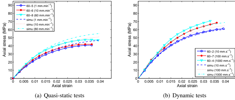
Figure 4.43: Comparison of experimental and numerical data for tests of 60^\circ specimens of PP-30GF
