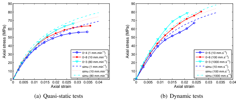
Figure 4.46: Comparison of experimental and numerical data for tests of 20° specimens of PP-40GF
