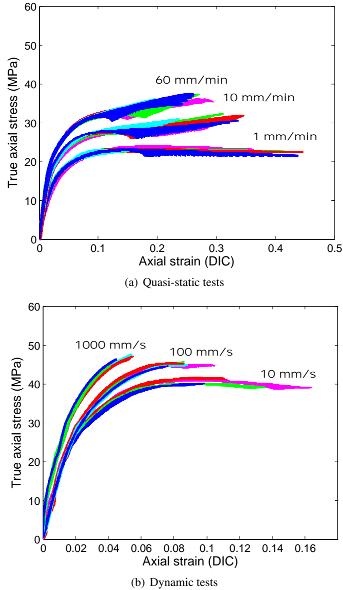
Figure 4.9: Quasi-static and dynamic tensile behaviour of PP, as measured by DIC
