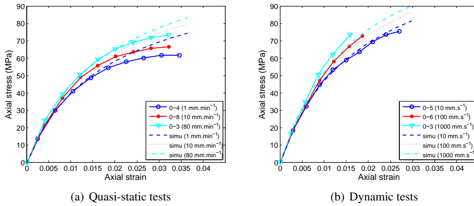
Figure 4.45: Comparison of experimental and numerical data for tests of 0° specimens of PP-40GF
