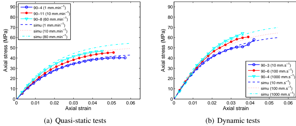
Figure 4.44: Comparison of experimental and numerical data for tests of 90^\circ specimens of PP-30GF
