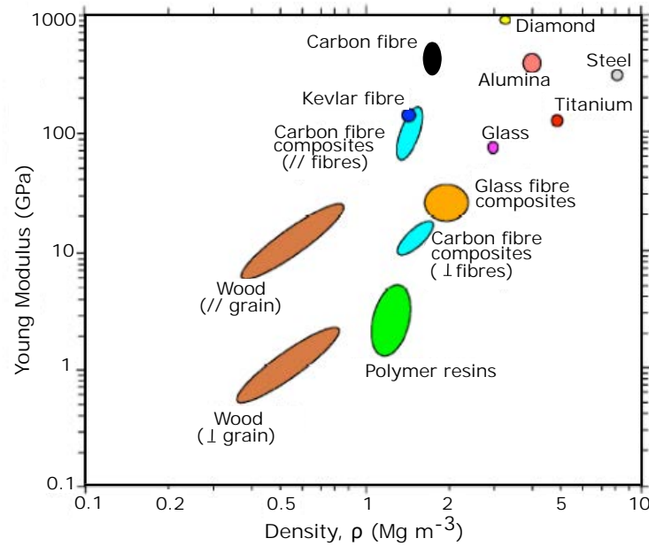
Figure 1.1: Stiffness of various materials with respect to their densities
