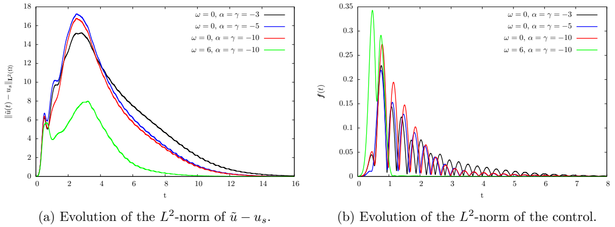
Figure 2.9 – Evolution of the L^2 -norm of \tilde{u} - u_s and f .
