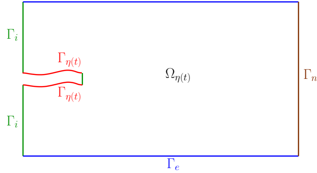
Figure 4.1 – Configurations of the fluid domain
