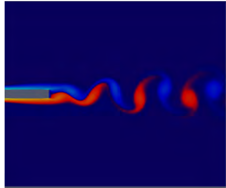
Vorticity of u at times t = 5.5 (without control).
