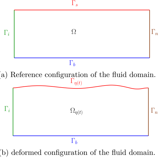
Figure 1.1 – Configurations of the fluid domain.
