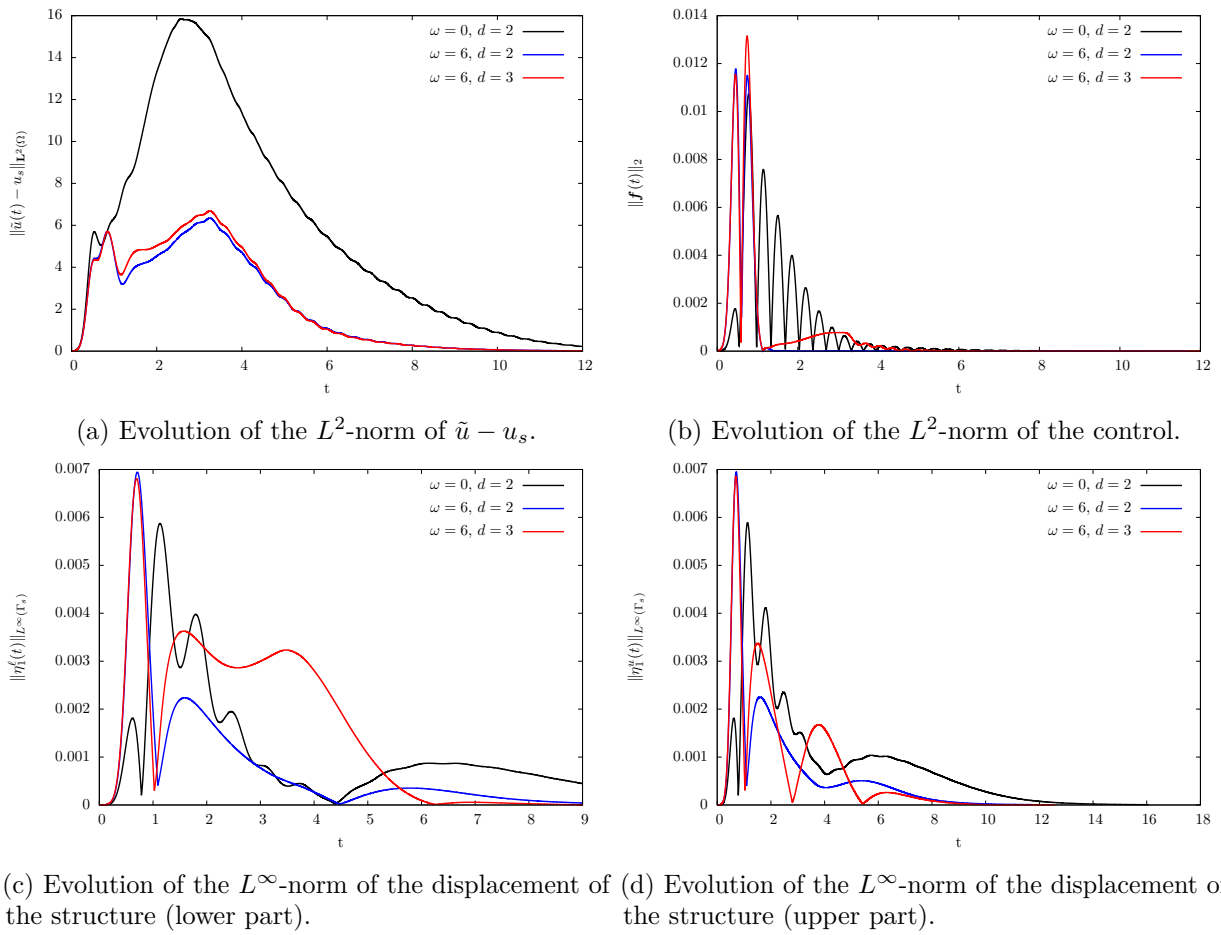
Figure 4.6 – Evolution of the L^2 -norm of \tilde{u} - u_s and \mathbf{f} , and the L^\infty -norm of \eta_1 of different controls ( \beta_{pert} = 0.1 ).
