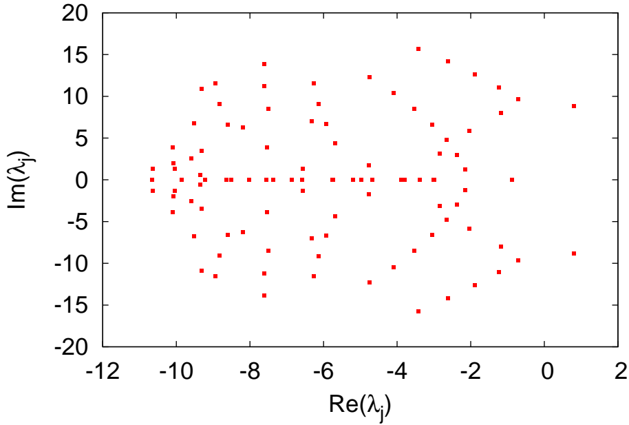
Figure 2.4 – Spectrum of the linearized Navier-Stokes operator for \text{Rey} = 200 .
