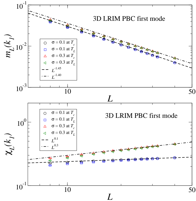
Figure C.8: FSS in the magnetisation sector for non-zero modes for the 3D LRIM with PBCs. In the top image the first magnetisation mode clearly scales as m_L^\dagger \sim L^{-(3-\sigma)/2} . In the bottom image the first susceptibility mode clearly scales as \chi_L^\dagger \sim L^\sigma . Both manifestly in favour of GFSS instead of the standard FSS.
