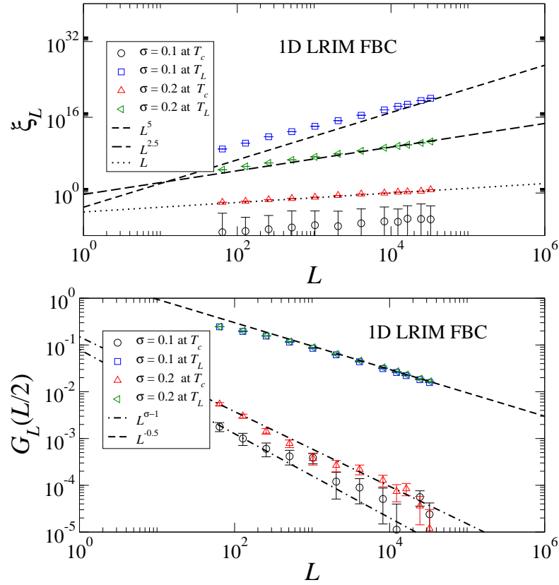
Figure 4.18: FSS for correlation sector for the 1D LRIM with FBCs. In the top image the correlation length scales close to \xi_L \sim L^\varrho at T_L and \xi_L^\dagger \sim L at T_c . In the bottom image the susceptibility clearly scales as G_L(L/2) \sim L^{-d/2} at T_L and roughly G_L^\dagger(L/2) \sim L^{\sigma-d} at T_c . Manifestly in favour of QFSS at T_L , and roughly GFSS at T_c .
