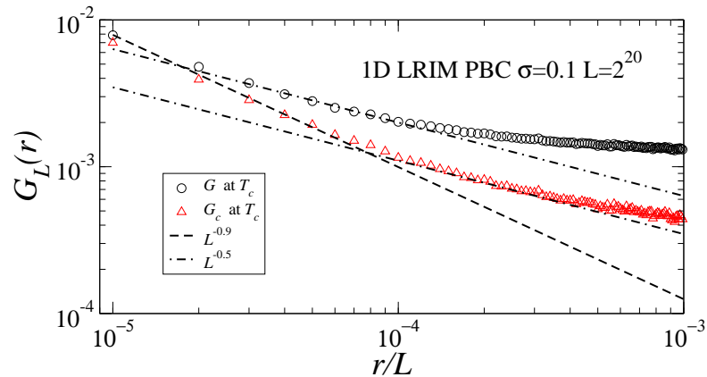
Figure 4.10: Correlation function in terms of distance for the 1D LRIM with PBCs. The dashed lines shows the QFSS and the Landau FSS respectively by L^{-0.5} and L^{-0.9} , one can observe a crossover between both of them. For short distances Landau FSS seems to dominate, but for intermediate distances QFSS seems to take over.
