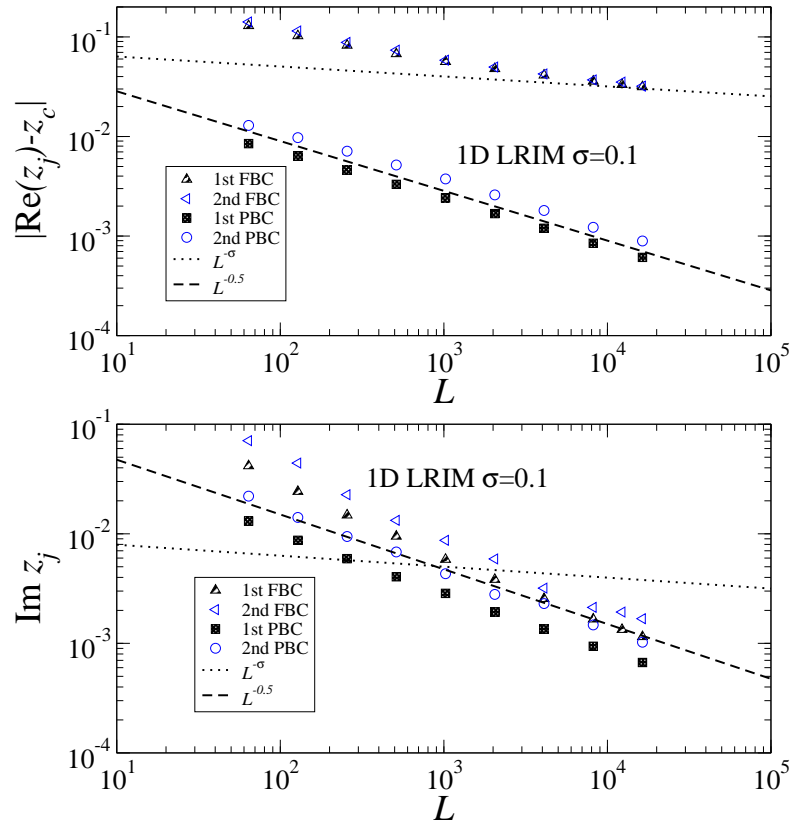
Figure 5.2: FSS for the first and second Fisher zeros for 1D LRIM with PBCs and FBCs for \sigma = 0.1 in terms of |\operatorname{Re}(z_j) - z_c| and \operatorname{Im}(z_j) .
