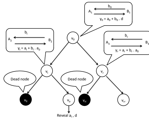
Figure 5.1: Pictorial view for an internal node of the Tree protocol. Here the coloring is such that c(v) = 1, c(v\ell) = 2, c(vr) = 3 .
