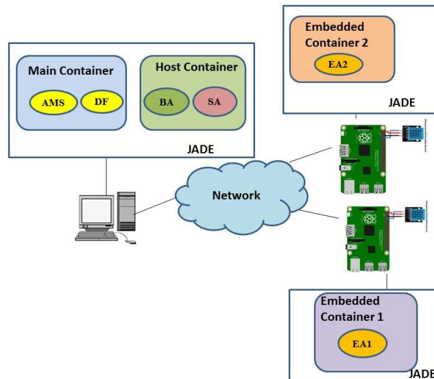
FIGURE 3.7: L'architecture MAPSO2++
