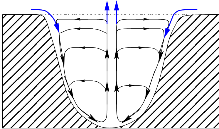
Figure II.10: Schematic of the circulation induced by downslope flow convergence over the valley centre at the beginning of the night, i.e. when a strongly stable stratified ground-based inversion layer has not developed yet. Arrows indicates the direction of the flow. Note that possible detrainment of downslope flows is not considered here. After Wagner [1932].
