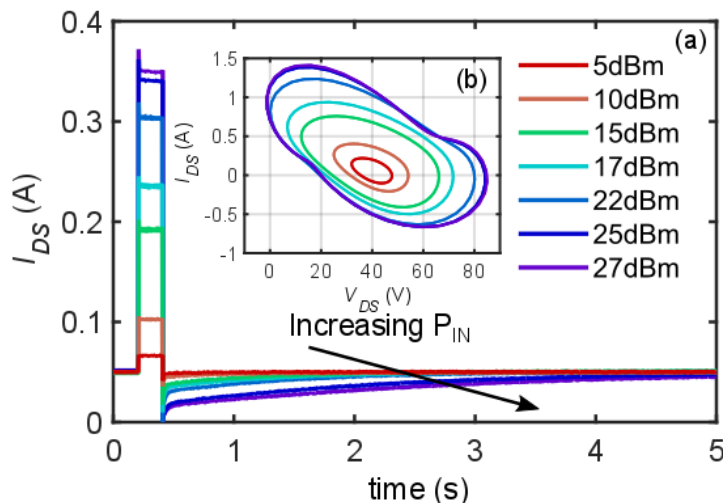
Figure 2-24: (a) Bias drain current measurements during single pulse excitation for fixed PW = 200 ms, Z_{LOAD\_maxPAE} and at 25^\circ\text{C} . While the time range measurement is 10 s, results are shown for a reduced time range to exhibit the linear shape of the pulses. (b) Corresponding extrinsic CW output load-lines derived from wave measurement at f_0 , 2f_0 and 3f_0 .
