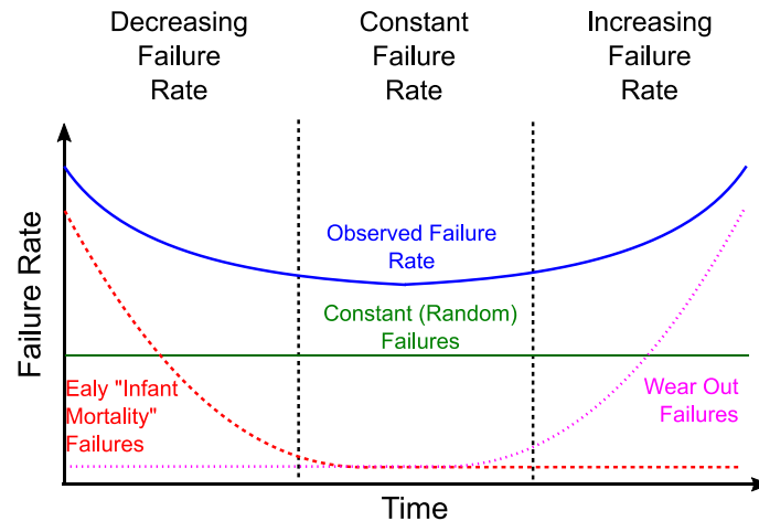
Figure 4-1: Bathtub curve describing the time dependence of failure rate for an electronic device.
