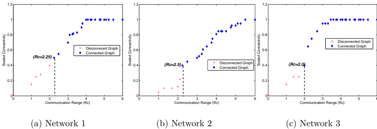
Figure 4.37: Scaled connectivity of networks versus different values of R_c
