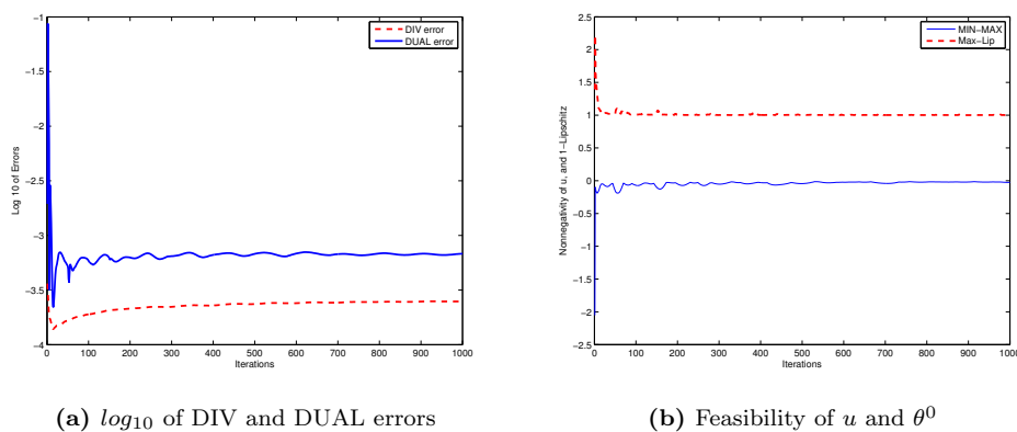
Fig. 3.5: Stopping criterion at each iteration
