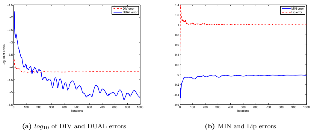
Fig. 5.4: Stopping criterion
