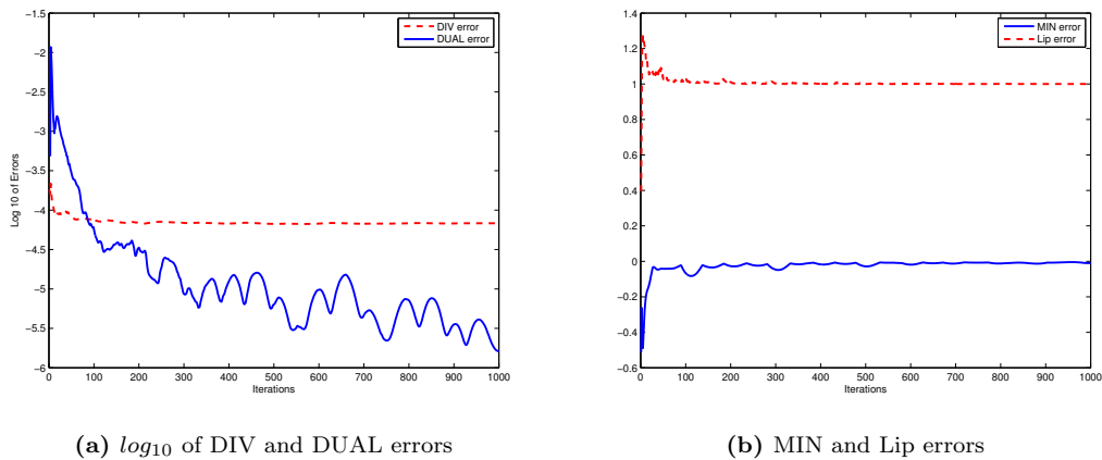
Fig. 5.6: Stopping criterion
