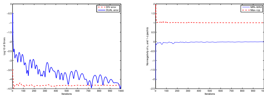
(a) \log_{10} of DIV and DUAL errors
