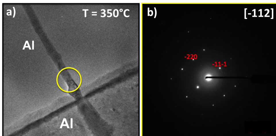
FIGURE 7.6: a) TEM image of a Ge NW completely transformed to Al after being heated in a furnace at 350^{\circ}\text{C} . b) A diffraction pattern on the transformed NW indexed as an FCC Al crystal oriented along the [-112] ZA.
