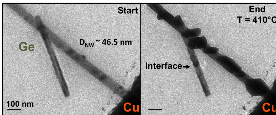
FIGURE 6.3: TEM images before and after heating at 410°C showing the propagation taking place in a Ge NW without been contacted to the Cu pad.
