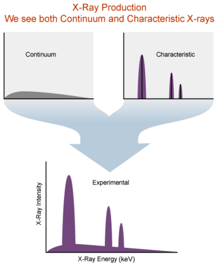
FIGURE 4.1: The X-ray spectrum displayed by the Energy Dispersive system comprises characteristic X-ray peaks superimposed on the continuum (Bremsstrahlung X-rays). [9].
