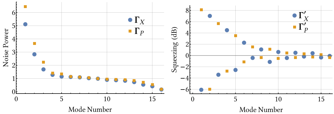
Figure 3.11: Left: Eigenvalues of \Gamma_X and \Gamma_P , in units of shot noise. Right: diagonal terms of \Gamma'_X and \Gamma'_P in dB for each mode of the common basis \{v'_n\} .
