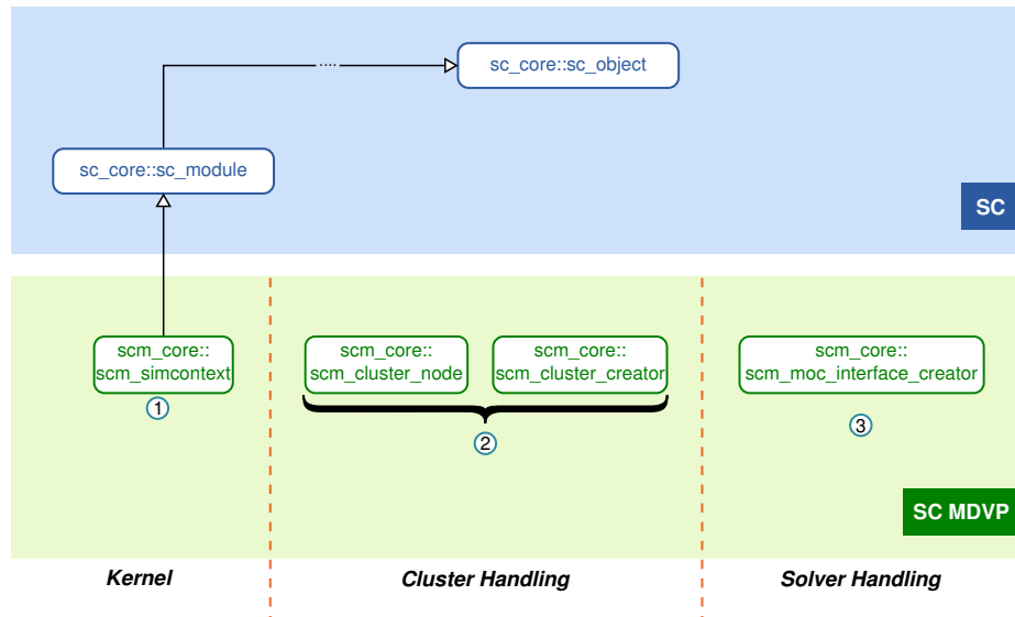
Figure 5.2: SystemC MDVP intrinsic classes
