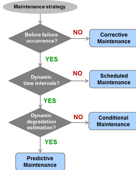
Figure 1.6. Maintenance strategies
