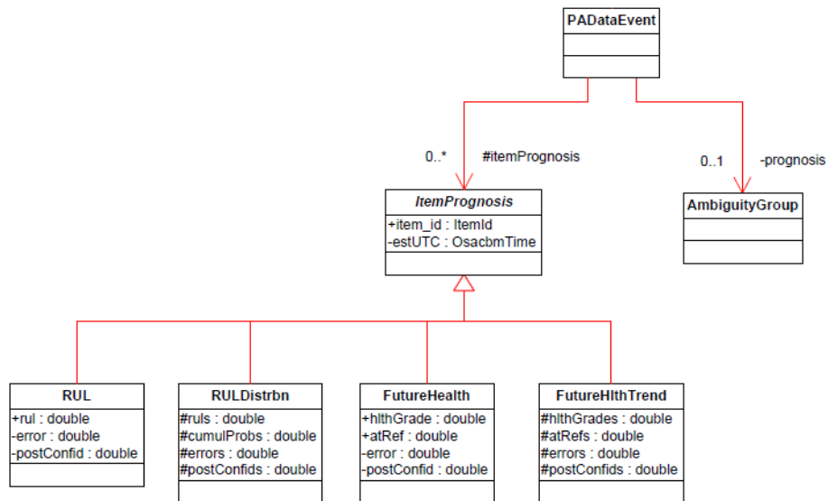
Figure 2.12 PADATAEvent data structure – OSA-CBM v 3.3.1
