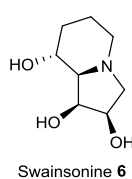
Figure 8 – Swainsonine.
