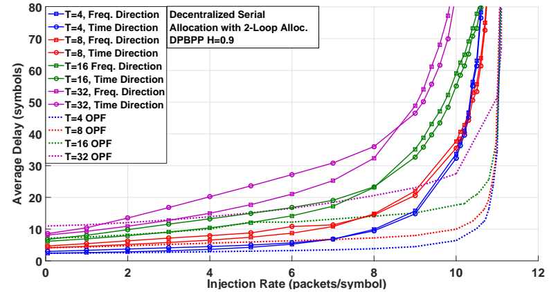
FIGURE 5.15: Average latency curves under non-uniform DPBPP traffic with increasing injection rate for centralized serial 2-loop allocation algorithm.
