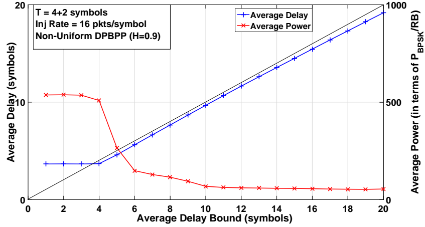
FIGURE 7.23: Resulting average delay and average power is shown with a 2-y plot, with T = 4+2 symbols, under non-uniform DPBPP traffic under an injection rate of 16 packets/symbol.
