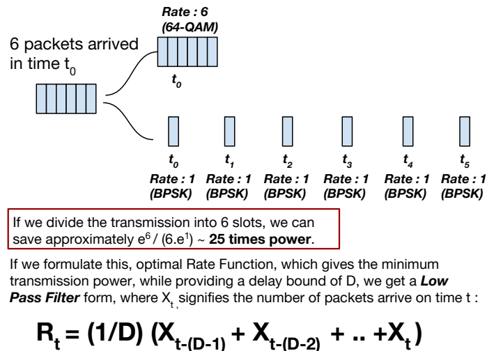
FIGURE 7.5: Maximum delay bounded rate scheduler can save substantial amount of power, as shown in this example
