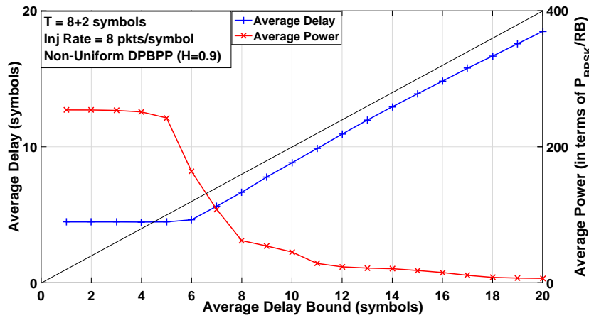
FIGURE 7.24: Resulting average delay and average power is shown with a 2-y plot, with T = 8+2 symbols, under non-uniform DPBPP traffic under an injection rate of 8 packets/symbol.
