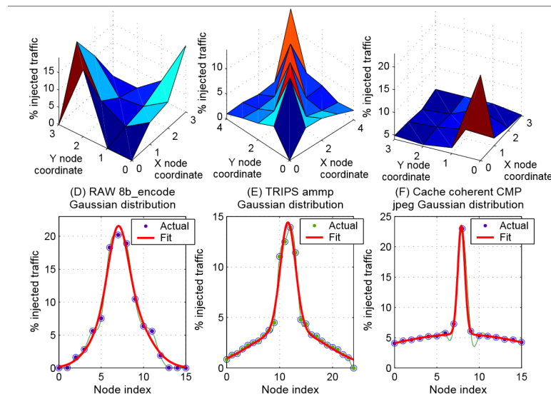
FIGURE 2.13: Gaussian normal distribution fits well for 3 different applications under different cache coherency protocols and CMP architectures. (Image taken from [8])
