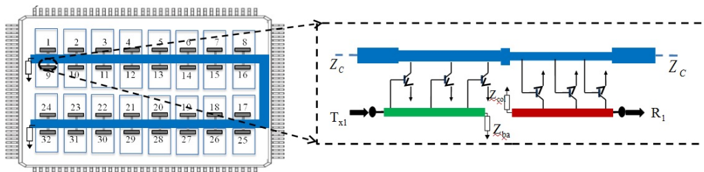
FIGURE 3.11: Proposed access via transistor mechanism for WiNoCoD (Image taken from [80]).
