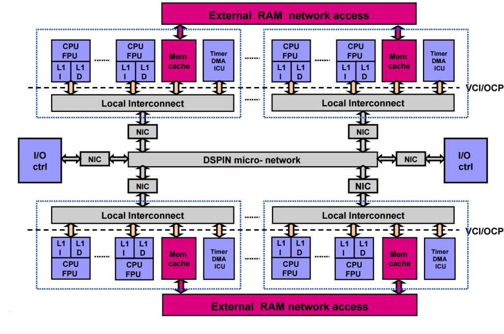
FIGURE 2.5: TSAR's tiled architecture and distributed memory
