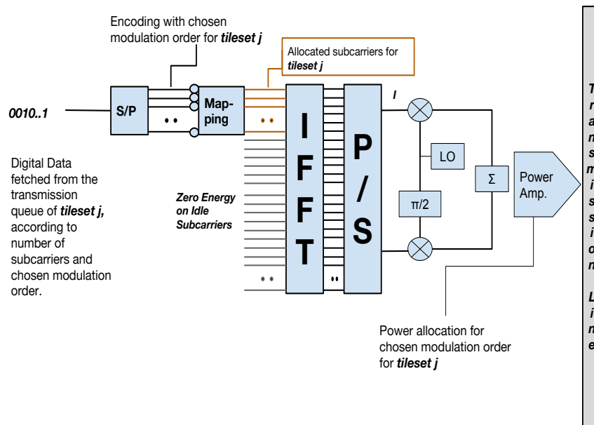
FIGURE 7.3: Transmission power tuning for the chosen constellation order
