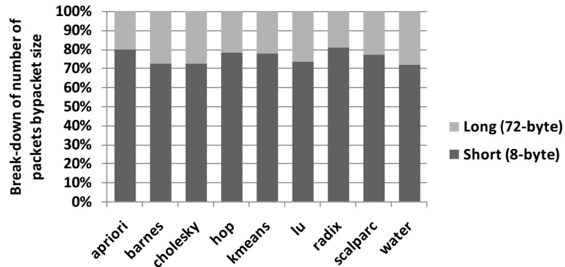
FIGURE 2.14: Percentages of short and long packets for various PARSEC benchmark applications (Image taken from [62]).
