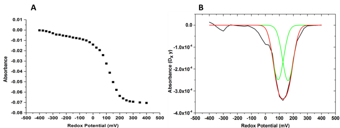
Figure 16 Potentiometric titration of wild type cNOR with DDM (2 nd batch) at pH 7.5, A) Absorbance values from Soret band, B) Gaussian fitting of the first derivative of the absorbance values from Soret band
