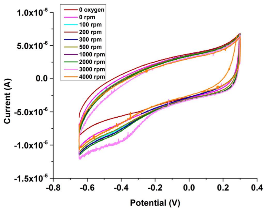
Figure 2. Cyclic voltammogram of quinone free bo_3 oxidase at pH 7.5 (Scan rate of 0.02 \text{ V.s}^{-1} )
