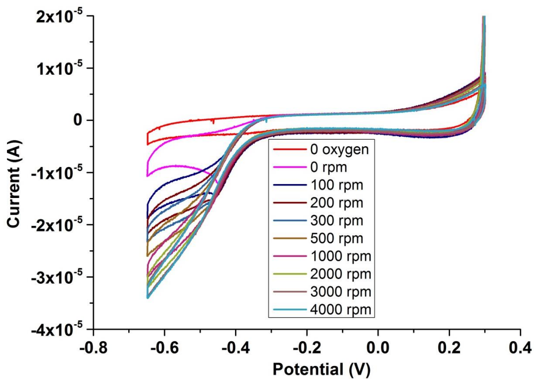
Figure 5. Cyclic voltammogram of Q101A at pH 7.5 (Scan rate of 0.02 \text{ V.s}^{-1} )
