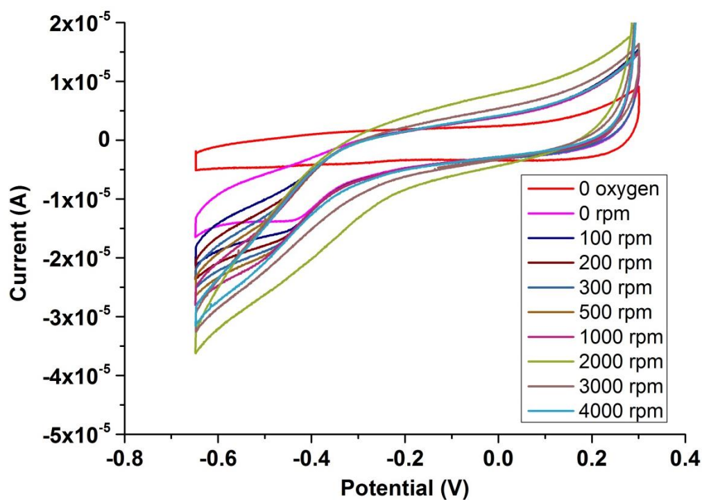
Figure 7. Cyclic voltammogram of Q101T at pH 7.5 (Scan rate of 0.02 \text{ V.s}^{-1} )
