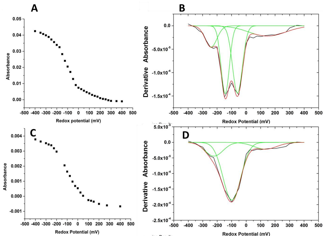
Figure 4.7 Potentiometric titration of wild type cytochrome bo_3 oxidase at pH 7.5, A) Absorbance values from Soret band, B) Gaussian fitting of the first derivative of the absorbance values from Soret band, C) Absorbance values from alpha band, D) Gaussian fitting
