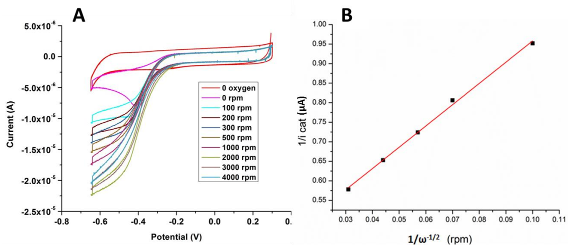
Figure 4.2 Cyclovoltammogram of wild-type cytochrome bo_3 oxidase at pH 7.5, B) Relation between the catalytic current and rotation rate of the electrode (Scan rate of 0.02 \text{ V.s}^{-1} ).
