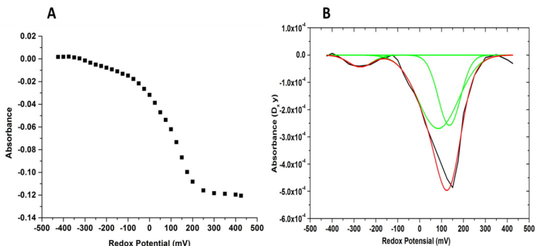
Figure 4.30 Potentiometric titration of wild type cNOR at pH 7.5, A) Absorbance values from Soret band, B) Gaussian fitting of the first derivative of the absorbance values from Soret band
