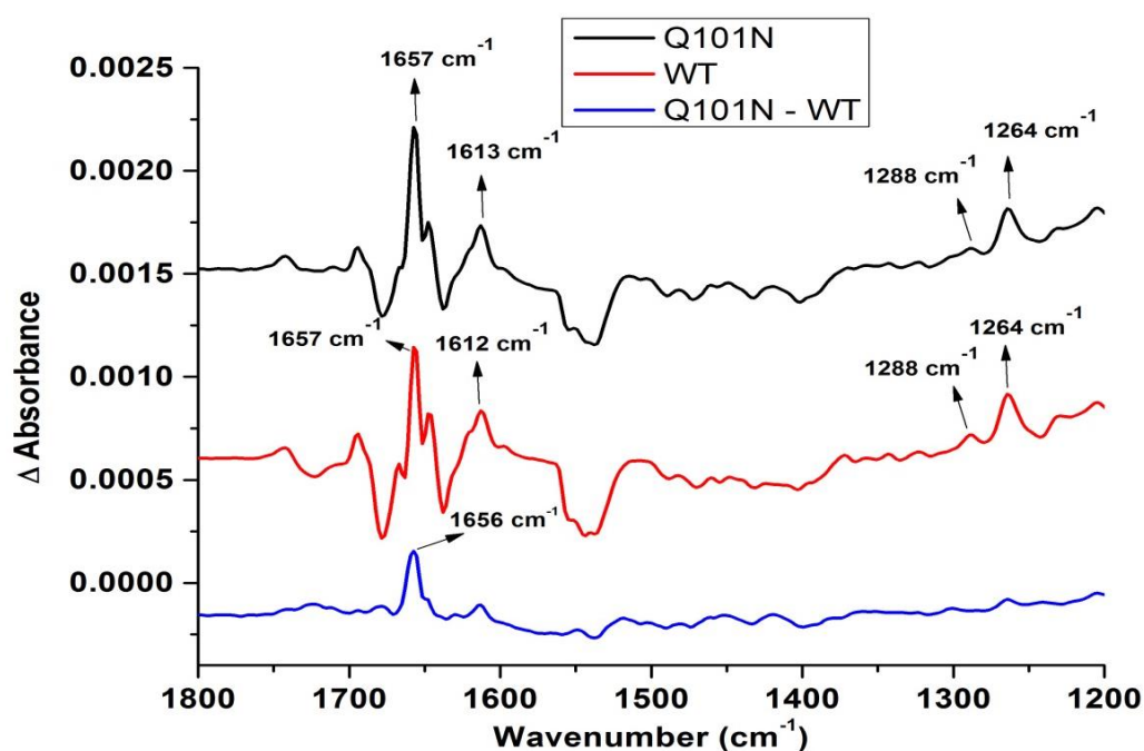
Figure 4.15 Oxidized-minus-reduced FTIR difference spectra of Q101N, wild-type cytochrome bo 3 oxidase and double difference spectrum of Q101N-WT at pH 7.5.
