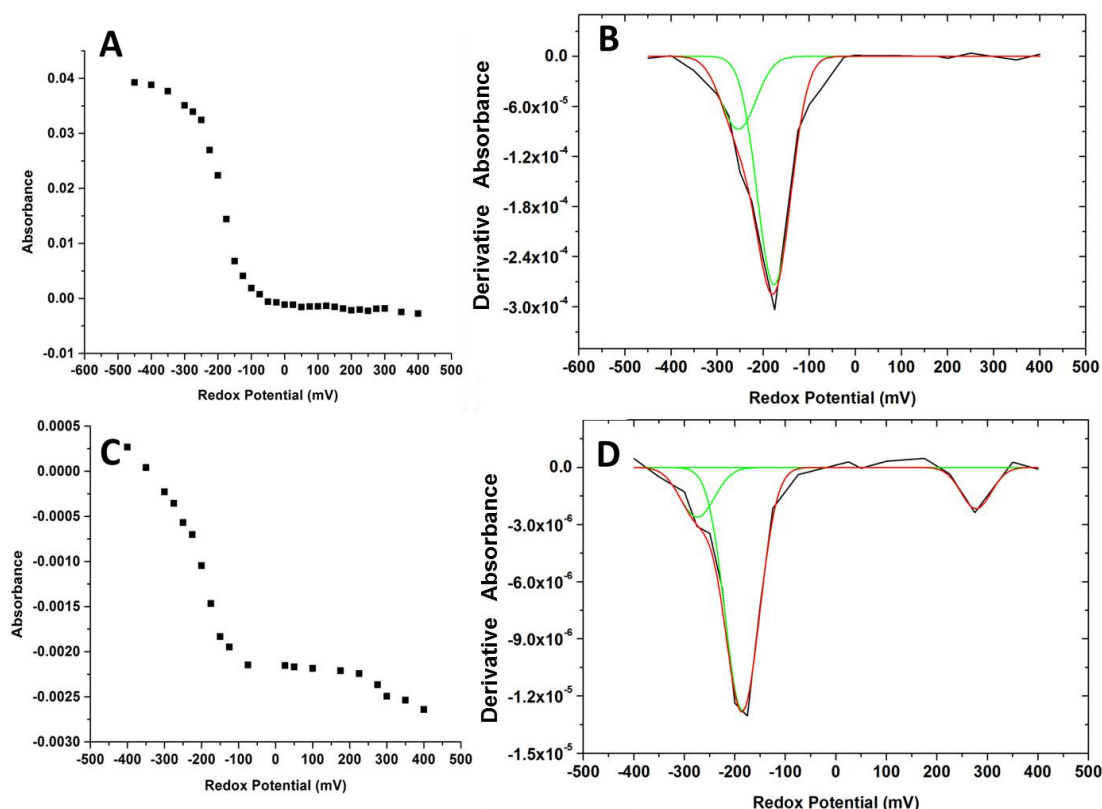
Figure 4.9 Potentiometric titration of cytochrome b_0_3 oxidase with menadione at pH 7.5, A) Absorbance values from Soret band, B) Gaussian fitting of the first derivative of the absorbance values from Soret band, C) Absorbance values from alpha band, D) Gaussian fitting of the first derivative of the absorbance values from alpha band
