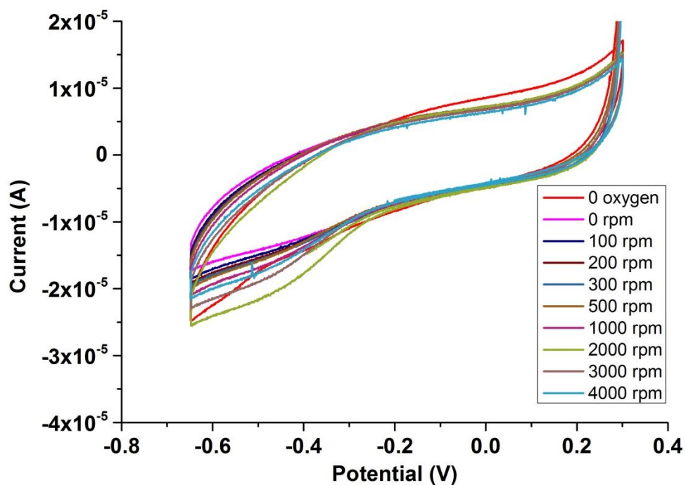
Figure 8. Cyclic voltammogram of I102N at pH 7.5 (Scan rate of 0.02 \text{ V.s}^{-1} )
