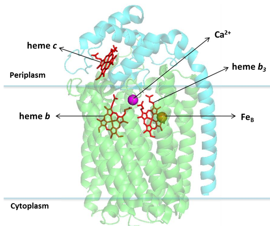
Figure 4.27 Structure of cNOR from P. aeruginosa . (3WFB.pdb)
