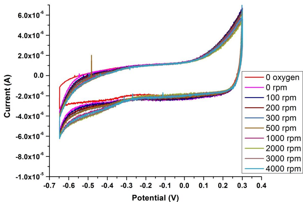
Figure 6. Cyclic voltammogram of Q101L at pH 7.5 (Scan rate of 0.02 \text{ V.s}^{-1} )
