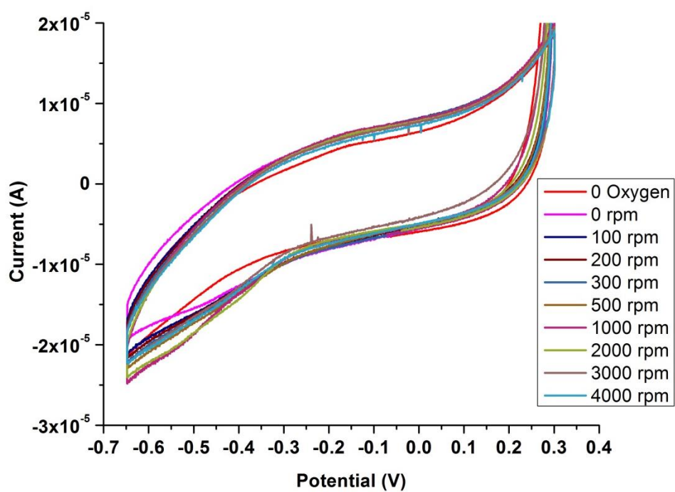
Figure 4. Cyclovoltammogram of Q101N at pH 7.5 (Scan rate of 0.02 \text{ V.s}^{-1} )
