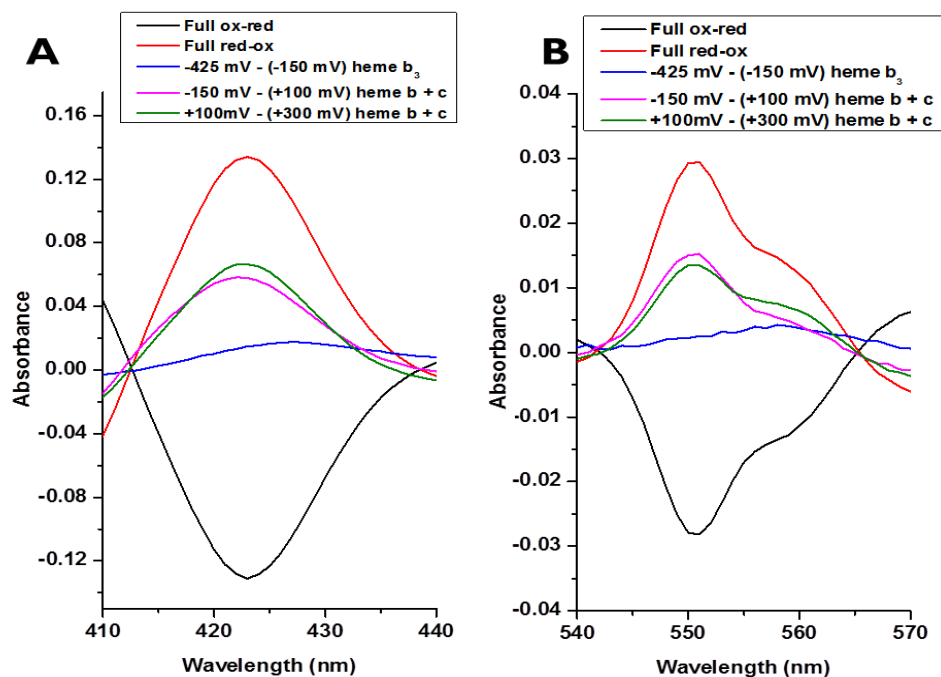
Figure 20 Investigation of the potentiometric titration of wild type cNOR (1 st batch) by steps, A) Soret band B) alpha band at pH 7.5.
