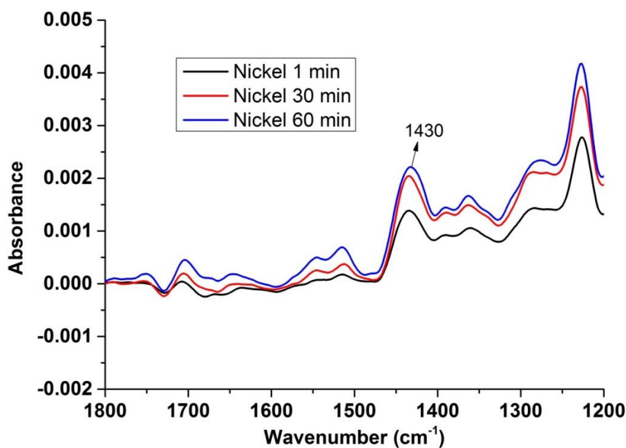
Figure 4.24 SEIRA spectra of the \text{Ni}^{2+} coordination of NTA at different times after the addition of \text{NiSO}_4 solution
