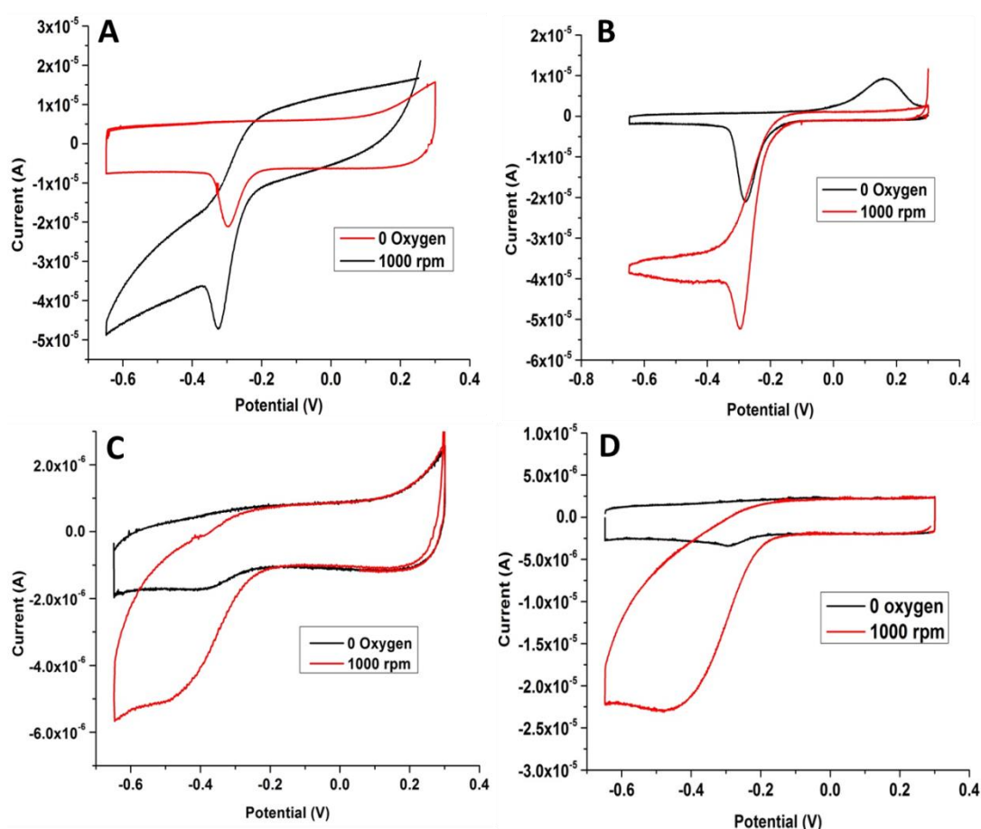
Figure 4.6 Cyclovoltammogram of A) bo_3 + Q_1 B) bo_3 + Q_2 C) bo_3 + Q_{10} D) bo_3 + menadione at pH 7.5 (scan rate of 0.02 \text{ V.s}^{-1} )
