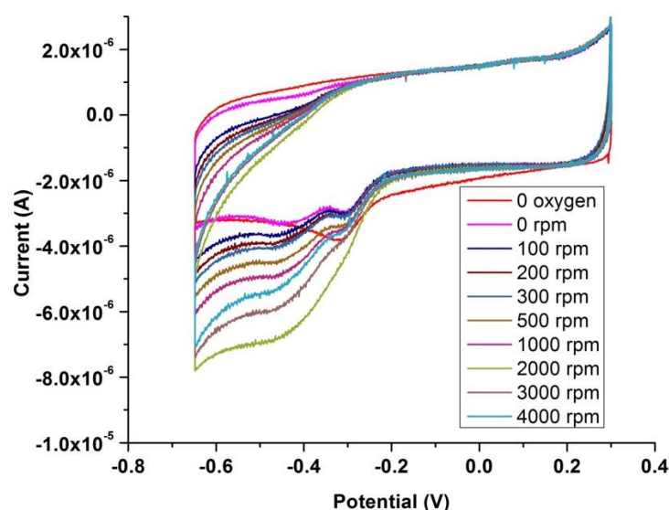
Figure 4.3 Cyclic voltammograms of K362M mutant of cytochrome bo 3 oxidase at pH 7.5 (Scan rate of 0.02 V.s -1 )
