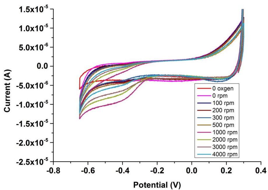
Figure 11. Cyclic voltammogram of quinone free D75N at pH 7.5 (Scan rate of 0.02 \text{ V.s}^{-1} )
