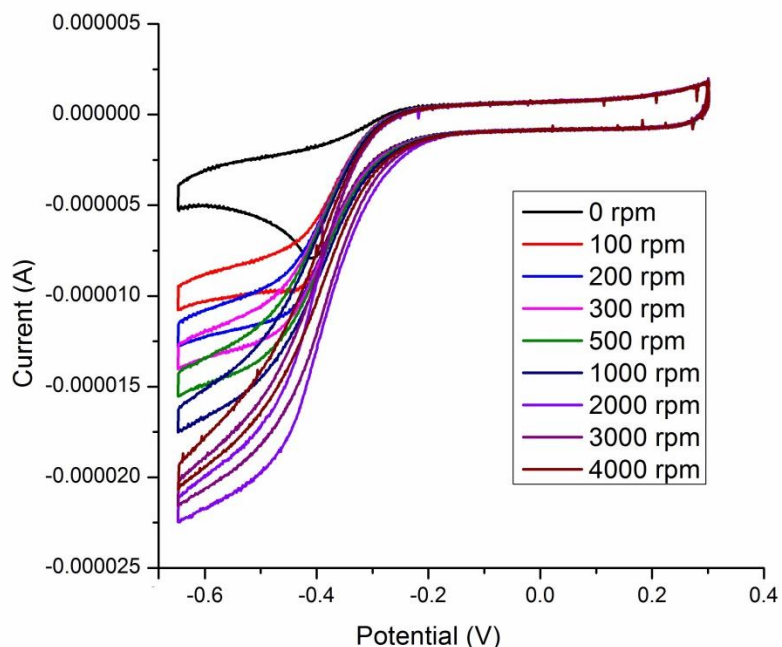
Figure 2.5 Cyclic voltammogram of cytochrome bo_3 oxidase immobilized on a rotating gold disk electrode (in KPi buffer at pH 7.5) modified with Au nanoparticles and thiols ( 0.02 \text{ V.s}^{-1} ).
