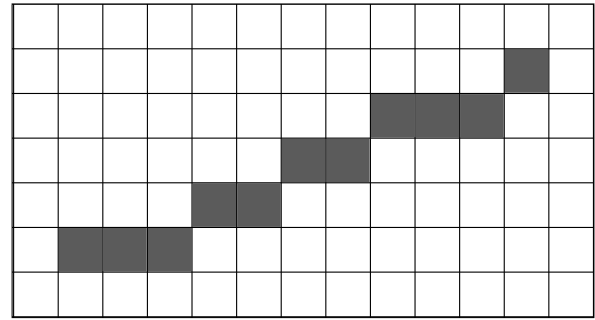
(b) segment naïf D(3, 7, 0, 7)
