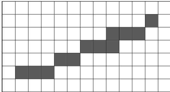
(c) segment *-connexe D(3, 7, 0, 8)
