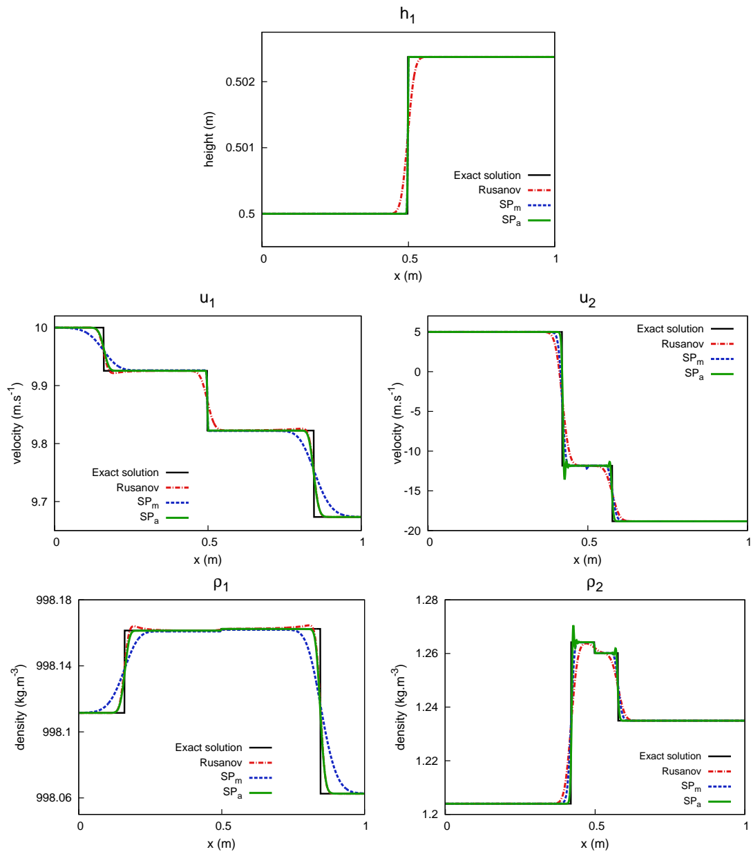
Figure 3.8: Approximate solution for test case 2 at T = 23.10^{-5} s with 1000 cells.
