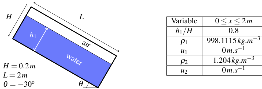
Figure 4.13: Initial conditions for the pipe filling test case.
