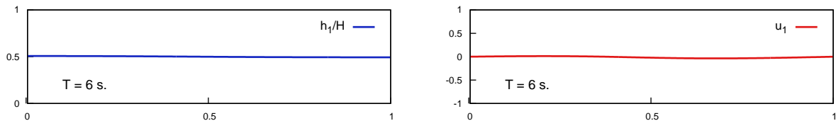
Figure 5.9: h_1 and u_1 fields at T = 6 s for H = 10 m and v_{max} = 0.5 .
