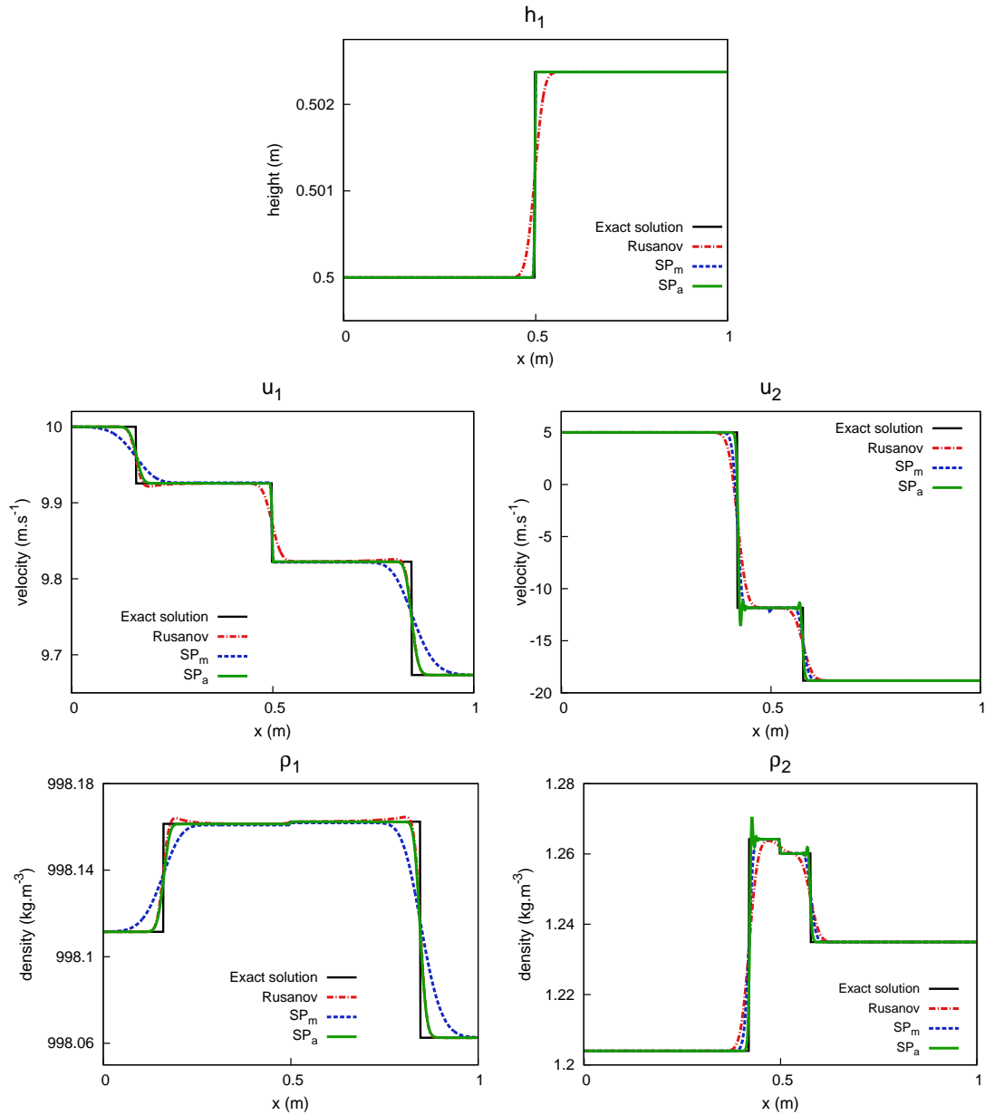
Figure 3.8: Approximate solution for test case 2 at T = 23.10^{-5} s with 1000 cells.
