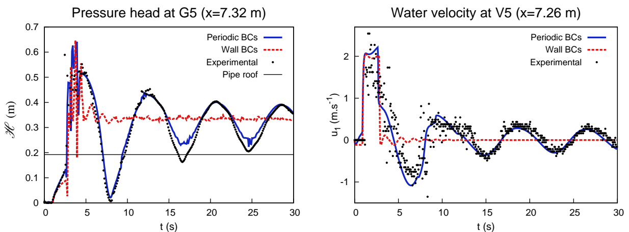
Figure 6.14: Influence of air pocket entrapment through the choice of boundary conditions (300 cells, c_{1,ref} = 300m.s^{-1} ).
