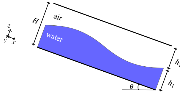
Figure 6.22: Geometric description for sloped pipes.
