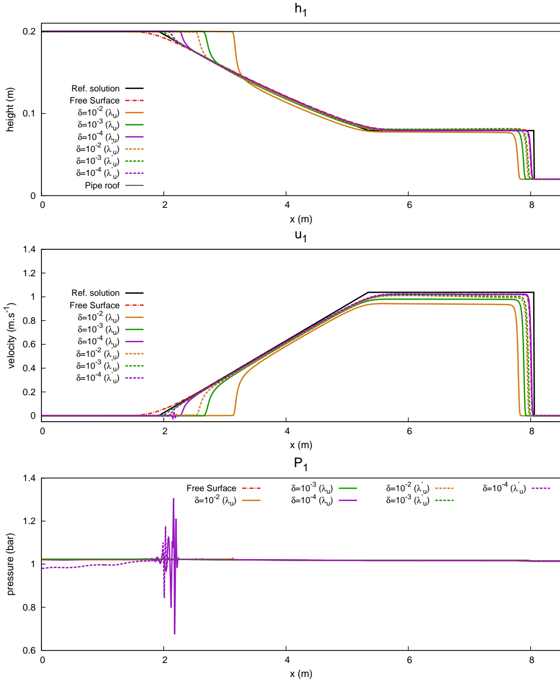
Figure 4.12: Influence of the threshold value and the velocity relaxation parameter for the pressurized dambreak problem (1000 cells, t = 2.2s ).
