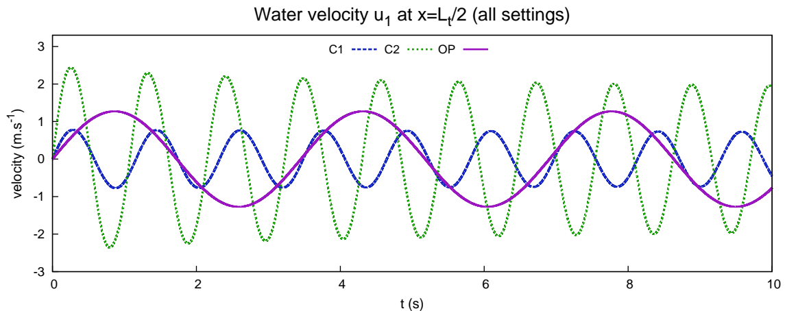
Figure 6.21: Comparison of the water velocity between the different settings using the CTL model with 300 cells.
