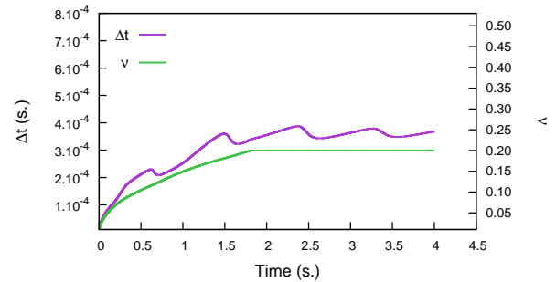
Figure 5.5: \Delta t and v in function of time for H = 1\text{ m} and v_{\max} = 0.2 .
