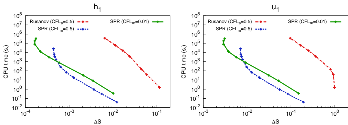
Figure 4.9: Deviation in L^1 -norm against CPU time for the dambreak problem.
