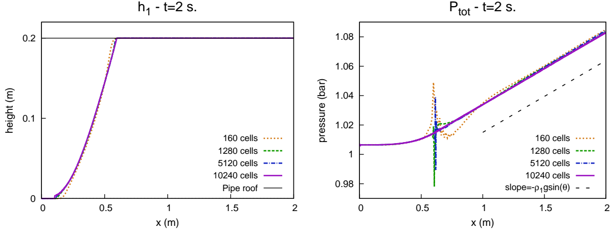
Figure 6.5: h_1 and P_{\text{tot}} = \frac{1}{H}(h_1 P_1 + h_2 P_2) at t = 2 s.
