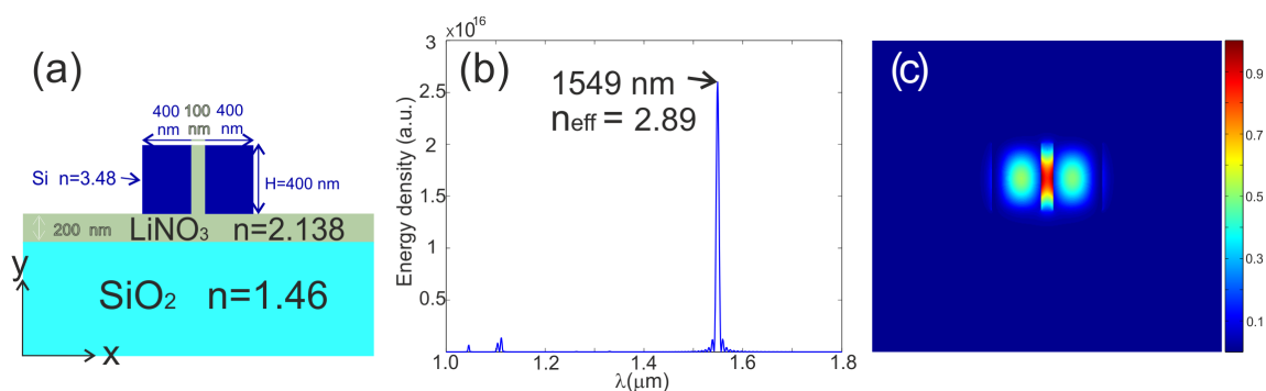
FIGURE 2.2 – (a) Schematic cross-section of the slot WG considered in the FDTD mode calculation window. The calculation window size is 590 \times 490 in the xy cross section, and a uniform meshing of d_x = d_y = 5 nm is employed. (b) Energy density spectrum. (c) Normalized electric field amplitude x component of the calculated mode profile.
