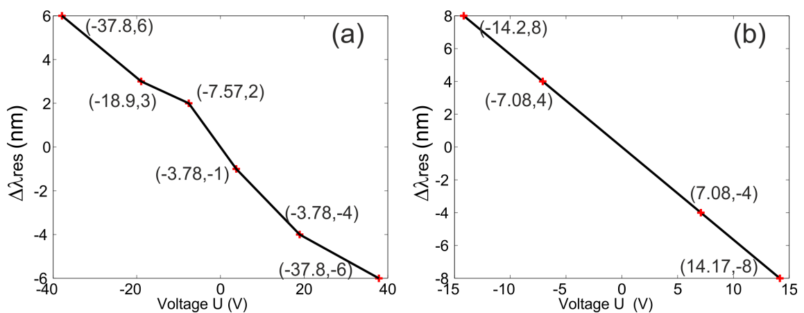
FIGURE 3.28 – \Delta\lambda_{res} versus voltage applied on the 1 \mu\text{m} separation of planar electrodes on slot Bragg gratings with parameters of a = 380 nm, W_{air} = 260 nm, W_{si} = 200 nm, W_s = 100 nm, number of air grooves on each side of defect N=7 (a) W_d = 360 and H=500 nm. (b) W_d = 340 nm and H=700 nm.
