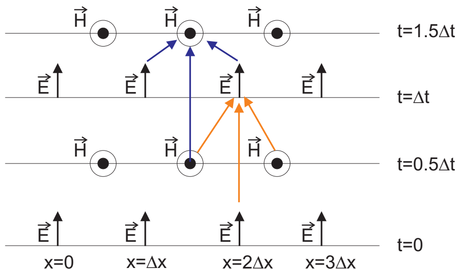
FIGURE 2.7 – Space time chart of the Yee algorithm for a 1D wave propagation example showing the use of central differences for space derivatives and leapfrog for the time.
