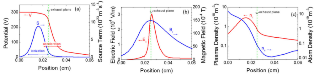
Figure 1.8 – Axial distributions of time averaged (a) plasma potential and ionization rate, (b) external radial magnetic field and axial electric field, (c) plasma density and xenon atom density, from a 2D hybrid model of a Hall thruster (SPT100 type, xenon mass flow rate 5 mg/s, applied voltage 300 V) [14, 13].
