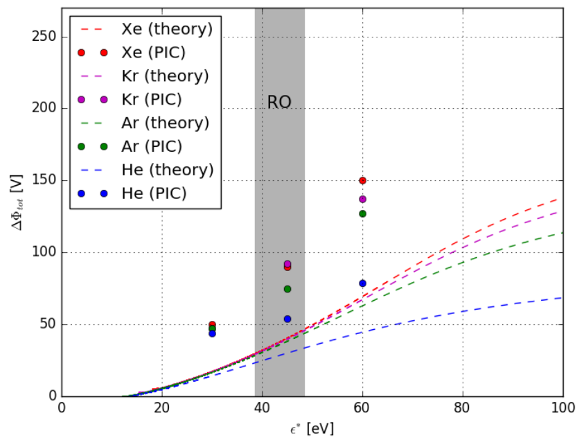
Figure 7.8 – Evolution of the plasma potential drop at the walls at steady state as a function of \epsilon^* : (dashed lines) theoretical results from the global model, (dots) PIC/MCC results. Each color corresponds to a given propellant: (red) xenon, (blue) helium, (green) argon, and (purple) krypton. The range of \epsilon^* for which ROs are observed is highlighted by a light gray rectangle.
