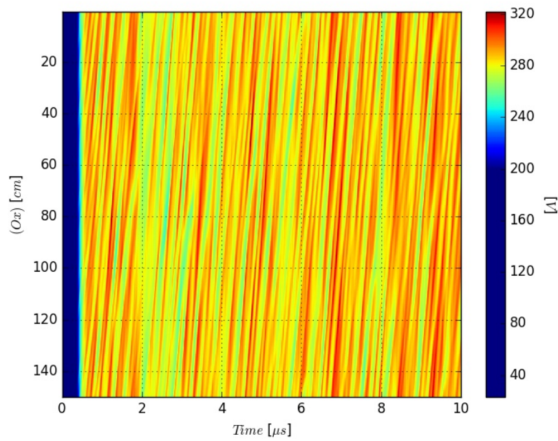
Figure 4.4 – Time evolution of the plasma potential profile taken from 1D cuts of the 2D (Ox - Oy) simulation domain taken along (Ox) , at y = L_y/2 . Collisions are “turned on” with parameters from Table 3.3. The color-bar has been rescaled in order to highlight the instability behavior.
