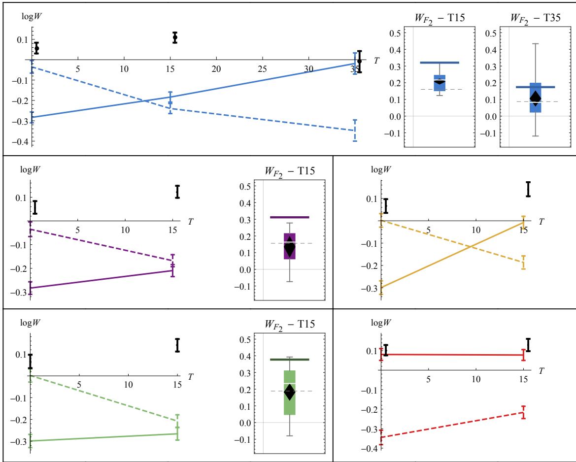
Figure 3.6: Fitness analysis of autodiploids parents, F1 and F2 diploid hybrids. Colors are the same as in Figure 3.5. Graphs represent the logfitness trajectories of homozygous diploid parents (Solid lines, autodiploids from haploid MATa , Dashed lines, autodiploids from haploid MAT\alpha ) and the logfitness of F1 hybrids (black dots). Error bars represent the standard error. Note that in all lines but P3 (red curve), the MATa parent is also ade2\Delta . Box plots present the logfitness distribution in F2 hybrids relative to mean parental logfitness. Diamonds represent F2 hybrids mean relative fitness and its interval confidence (95%). F1 hybrid fitness (darker bars), and the average between F1 and parents mean fitness (grey dashed bar) are plotted for comparison.
