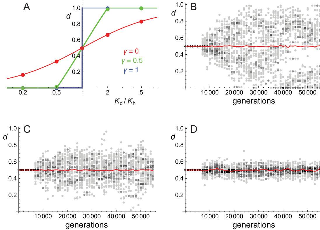
Figure 1: A, Evolutionarily stable strategy rate of diploidy ( d_{eq} ) as a function of the ratio of carrying capacities K_d/K_h , and for different levels of differentiation between phases ( \gamma_{ah} = \gamma_{hd} = \gamma ). Lines, analytical prediction in the absence of deleterious mutations (eq. [15]). Circles, multilocus simulations in the absence of deleterious mutations. Blue, \gamma = 1 ; green, \gamma = 0.5 ; red, \gamma = 0 . B–D, Distribution of alleles present at the modifier locus throughout the simulation, in the absence of deleterious mutation, with K_d = K_h = 15,000 , r_d = r_h = 1.8 , and \gamma_{hd} = \gamma_{dh} = 0.5 . Shading corresponds to the frequencies f of different ranges of values of d in the population, from light gray to black: f \in [1\%, 5\%] , f \in [5\%, 10\%] , f \in [10\%, 20\%] , and f \geq 20\% . B, When the environment stays constant, a large range of values of d is maintained in the population. C, Fluctuations of the relative sizes of the haploid and the diploid niches of low amplitude ( \lambda = 1/15 , \tau = 4 ) narrow this range. D, Increasing the amplitude of fluctuations ( \lambda = 1/2 , \tau = 4 ) further narrows the range around the ESS value of d . In all cases, the average value of d in the population stays near 0.5 (red lines).
