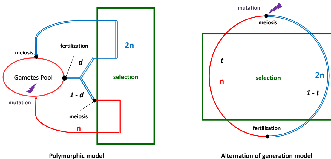
Figure 5: Polymorphic and alternation of generation models
