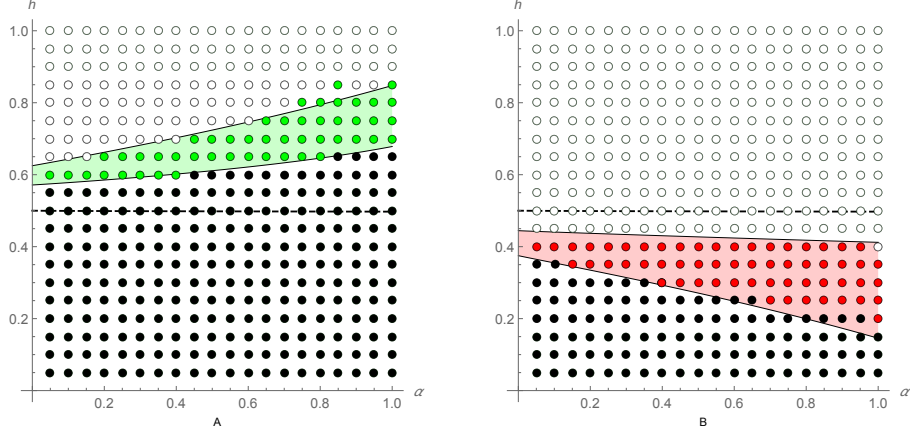
Figure 1.5: Parameter space where haploidy, diploidy and haploid-diploid life cycles are favoured where the relative strength of selection in haploids compared to homozygous diploids( \alpha ) and dominance h vary. Background colors: prediction from the two-locus stability analysis extrapolated to multiple loci. Circles: multilocus simulation results starting from three different initial haploidy rates ( d_{init} = 0.01, 0.5 , or 0.99 ), with population size 20,000. White: evolution toward haplonty. Green: convergence stable haploid-diploid life cycles. Red: either haploidy or diploidy is favoured, with a repelling state in between. Black and gray: evolution toward diplonty. (A): Diploids have higher intrinsic fitness ( S_h = 0, S_d = 0.025 ) and (B): haploids have higher intrinsic fitness ( S_h = 0.025, S_d = 0 ) Map length: R = 100 . The dashed lines show where haploidy (above dashed lines) and diploidy (below dashed lines) are favoured when there is no difference in intrinsic fitness ( S_h = S_d = 0 ). Mutants change the life cycle by a small amount ( |\delta| = 0.002 ) and the genome-wide haploid mutation rate, U = 0.1 .
