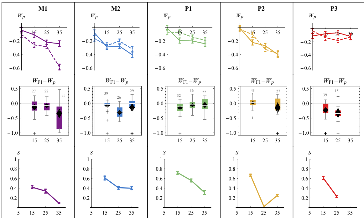
Figure 3.5: Reproductive isolation analysis at transfer 15, 25 and 35 (x-axis) in five MA3 line pairs (columns). Two pairs of mutator lines (M1 and M2) are msh2Δ and 3 pairs of mutator lines (P1, P2 and P3) are pms1Δ . The upper panels display parental competitive logfitness trajectories, where the solid curve represents the MAT \alpha parent and the dashed curve the MAT \alpha parent. Error bars show the standard error of the fitness estimations. The middle panels represent the relative competitive logfitness of the haploid F1 segregants, shown in Tukey Boxplot (parents have W = 0 ). Diamonds represent F1 hybrids mean relative fitness and its interval confidence (95%). The number of hybrids analysed is displayed above the boxes. The lower panels show the mean spore survival ( S ) after crosses between haploid parents, and error bars represent the standard error.
