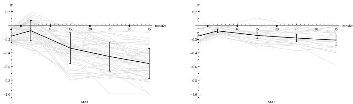
Figure 3.4: Competitive fitness trajectories of the haploid parental lines under treatment MA1 and MA3 treatment. The grey curves show individuals trajectories. The thick curves indicate the average fitness of the lines. Errors bars show standard deviation.
