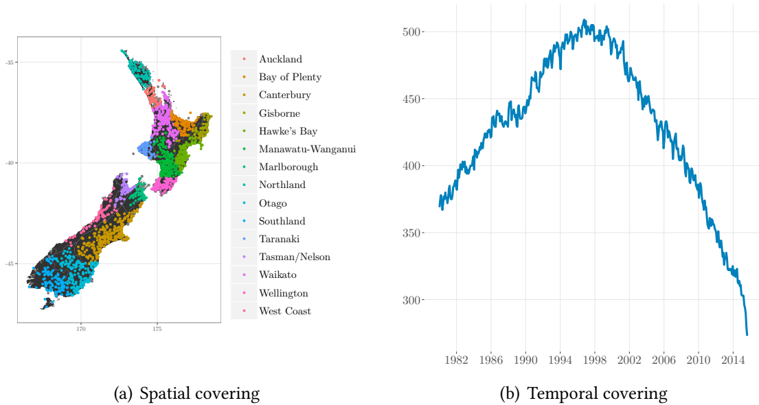
FIGURE C.2: Covering of Weather Stations Used to Construct the Soil Moisture Deficit Index
