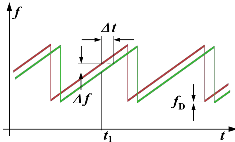
Figure 6 : principe de la modulation FMCW [1.11]
