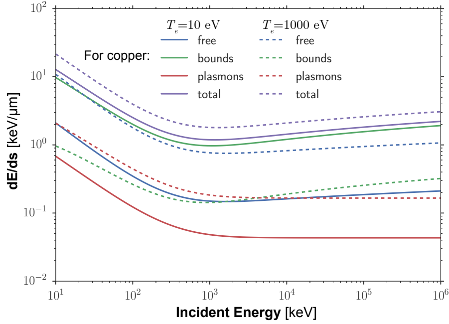
Figure 3.7 – Different contributions of the total stopping power in ionized copper at solid density. The solid lines correspond to T_i = T_e = 10 \text{ eV} while the dashed lines correspond to T_i = T_e = 1000 \text{ eV} .
