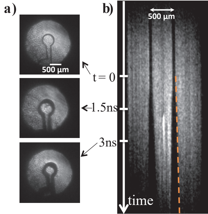
Figure 8.30 – Coil expansion inspected by optical shadowgraphy at \lambda = 532 \text{ nm} : a) optical gated images (0.65 ns window) from different shots and b) one shot streaked image (10 ns sweep window).
