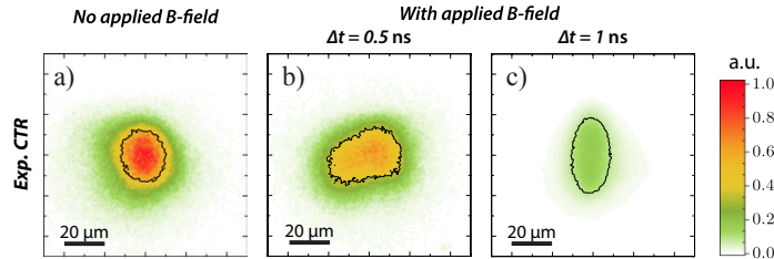
Figure 10.4 – Results of the experimental CTR imaging , for the two configurations i) target out of the coil plane and ii) target at the coil plane (see Figure 10.2), without imposed B-field and with imposed B-field (for the two delays \Delta t = 0.5 \text{ ns} and \Delta t = 1 \text{ ns} ), as labeled. The contour lines correspond to the half-height of the signals.
