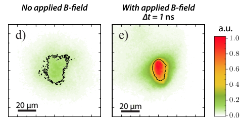
Figure 10.4 – Results of the experimental CTR imaging , for the two configurations i) target out of the coil plane and ii) target at the coil plane (see Figure 10.2), without imposed B-field and with imposed B-field (for the two delays \Delta t = 0.5 \text{ ns} and \Delta t = 1 \text{ ns} ), as labeled. The contour lines correspond to the half-height of the signals.
