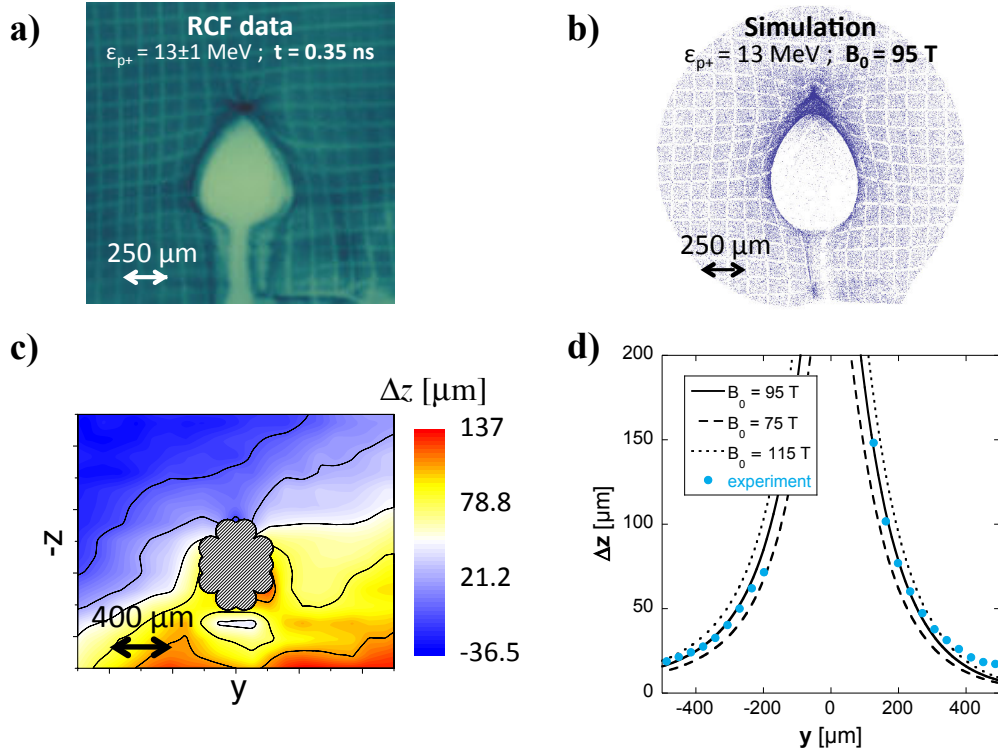
Figure 8.14 – a) Sample RCF image of proton-deflectometry measurement in an early probing time \Delta\tau = 0.35\text{ ns} after ns-laser light starts to irradiate the B-loop target's rear disk. The RCF position corresponds to the imprint of 13 \pm 1\text{ MeV} protons. b) 13 \pm 1\text{ MeV} proton imprint on detector plane given by a ballistic simulation of their trajectories over a 3D B-field map with B_0 = 95\text{ T} (previously calculated by the magnetostatic code). c) Map of experimental vertical deformations of the mesh shadow. The spatial scale on each image corresponds to the plane of the coil. d) Corresponding horizontal lineouts of the experimental (circles) and synthetic (curves, for different B-field strengths) vertical deformations of the mesh imprint.
