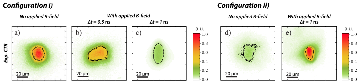
Figure 10.4 – Results of the experimental CTR imaging , for the two configurations i) target out of the coil plane and ii) target at the coil plane (see Figure 10.2), without imposed B-field and with imposed B-field (for the two delays \Delta t = 0.5 \text{ ns} and \Delta t = 1 \text{ ns} ), as labeled. The contour lines correspond to the half-height of the signals.
