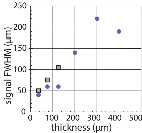
Figure 23.5 – Evolution of the rear-side self-emission with different Al target thicknesses, from experiments (in blue dots) compared with the results of PIC hybrid + CTR post-processor (grey squares). Original graph from [242].
