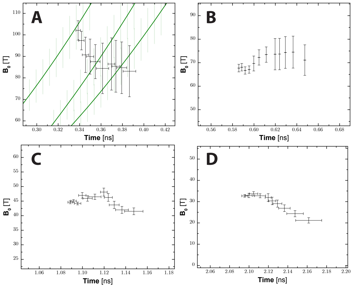
Figure 8.21 – Same as Figure 8.20 for the 2 nd experiment.
