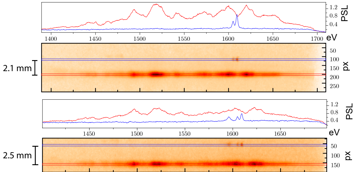
Figure 8.34 – top: Spectral emission of a Ni-coil target of the 3 rd experiment, with a secondary target at the coil vicinity containing a Cu-layer. bottom: Idem, but for a Ni-coil target of the 2 nd experiment. The combination of both images allows us to identify clearly the localization of the two observed emission lines of each image: more details are given in the text.
