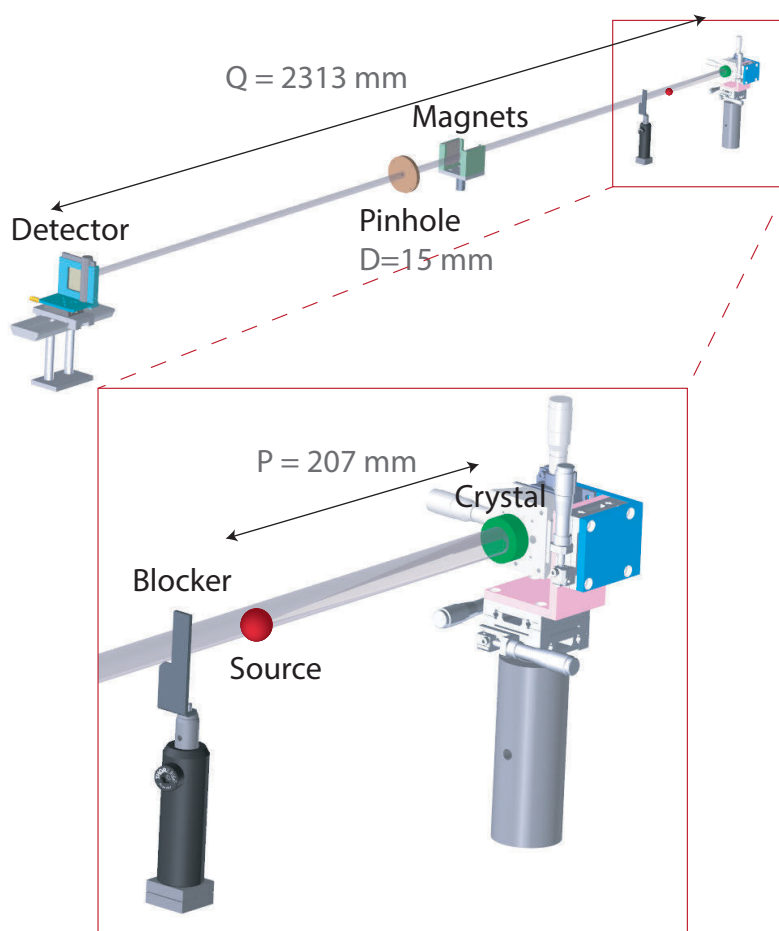
Figure 22.4 – Setup of the K_\alpha imager as used in our experiments.
