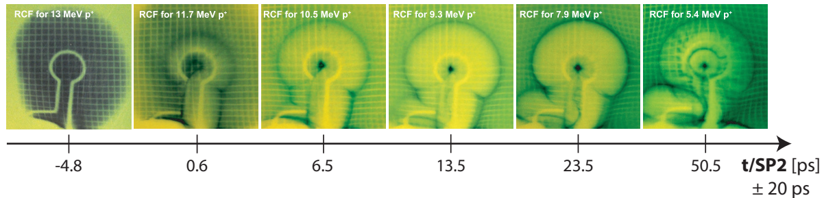
Figure 11.6 – Time-resolved build-up of the charge propagation and fields in the target's coil part as imaged by the RCF stack arrangement. t = 0 refers to the beginning of the SP1 interaction with the coil-target. The distance from Au foil to coil target is d = 5 mm. The absolute uncertainty on the delay of \pm 20 ps is due to the synchronization accuracy between SP1 and SP2 laser pulses.
