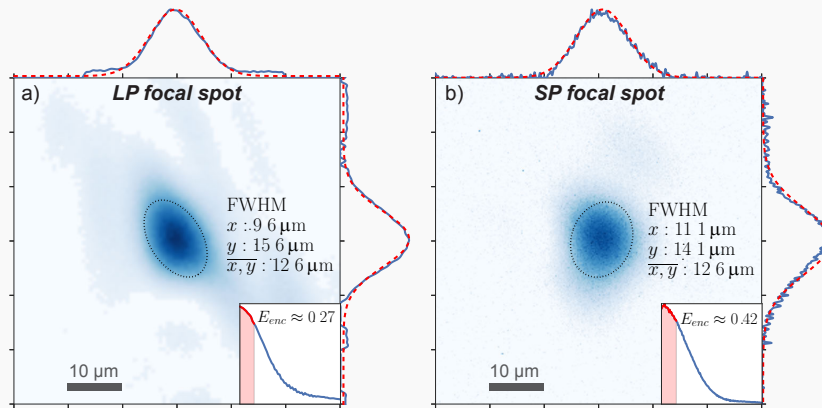
Figure 8.1 – Typical focal spot of a) LP laser beam and b) SP laser beam. The annotations of FWHM are obtained by a 2D gaussian fit. The insert is showing the azimuthally averaged radial profile with a 1D evaluation of the ratio of encircled energy over mean FWHM.
