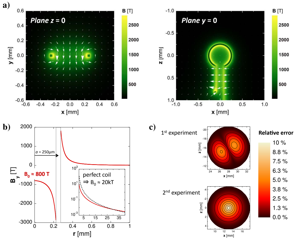
Figure 8.7 – Figure 3. a) 2D projections of the 3D Radia magnetostatic code extrapolation of the B-field produced by a a = 250\ \mu\text{m} capacitor-coil target for a circulating current I = 340\ \text{kA} : plane z = 0 on the left, plane y = 0 on the right (the coil center is at the frame origin). b) Corresponding axial component of the B-field against distance from the coil center, along the line between coil center and the B-dot probe position for the 1 st experiment, for a capacitor-coil target (solid red curve) and for a perfect coil of the same radius a (dashed black curve), for the same current. (c) Relative uncertainty of the B-field measurements by the B-dot probes at their positions, respectively in the 1 st (top) and the 2 nd & 3 rd (bottom) experiments.
