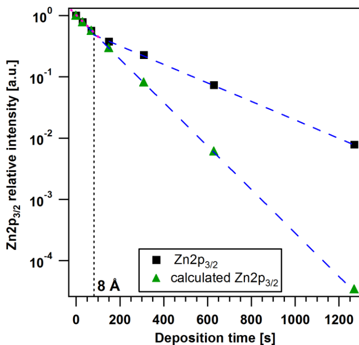
Figure 8.17: Normalized integrated \text{Zn}2p_{3/2} emission intensity versus \text{Ir}(\text{BPA}) deposition time. Below 70 \text{ s} the damping increases linearly (shown in the inset), indicating growth of a 8 \text{ \AA} thick monolayer. Above 70 \text{ s} the damping is exponential, which could suggest a layer-by-layer or island growth. The calculated damping of the \text{Zn}2p_{3/2} emission is also shown for a layer-by-layer growth considering the nominal \text{Ir}(\text{BPA}) deposition rate of 6.5 \text{ \AA}/\text{min} and a photoelectron escape depth of 13 \text{ \AA} .
