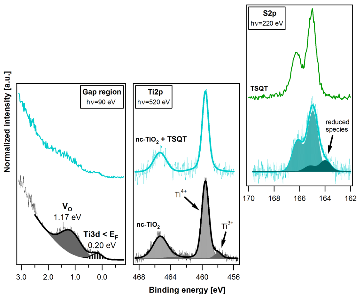
Figure E.5: Curve fitting analyses for the gap region, \text{Ti}2\text{p} and \text{S}2\text{p} emission spectra under synchrotron light irradiation. Due to higher surface sensitivity, the V_{\text{O}} and \text{Ti}3\text{d} < E_{\text{F}} gap states, \text{Ti}^{3+} \text{Ti}2\text{p} and reduced \text{S}2\text{p} emissions are clearly resolved. The quenching of the V_{\text{O}} gap and \text{Ti}^{3+} species in the nc- \text{TiO}_2 + TSQT composite layer is accompanied by the reduction of guest TSQT molecules as evidenced by the presence of \text{S}2\text{p} species with a smaller binding energy.
