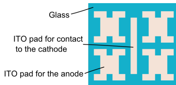
Figure 7.6: OLED grade, patterned ITO on glass substrate. This design yields 4 devices. The ITO strip located at the middle of the substrate is for contacting the cathode.
