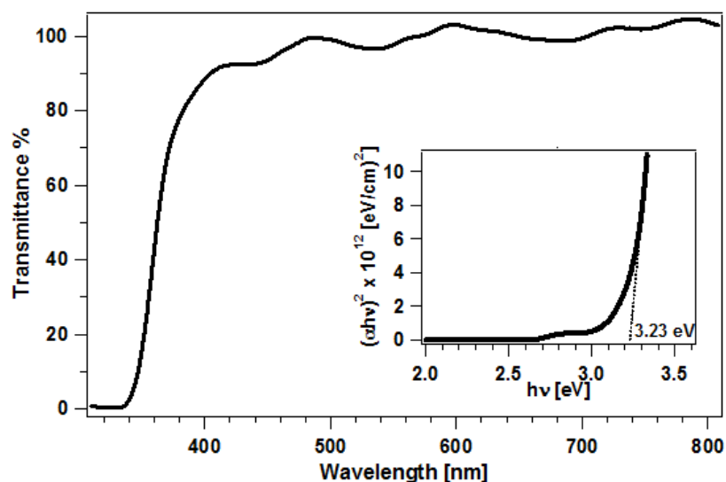
Figure 9.4: Optical transmission of the 2 μm thick anatase nc-TiO 2 film deposited on FTO glass substrate. Inset: An optical bandgap of 3.23 eV is derived from the plot, (\alpha h\nu)^2 versus h\nu .
