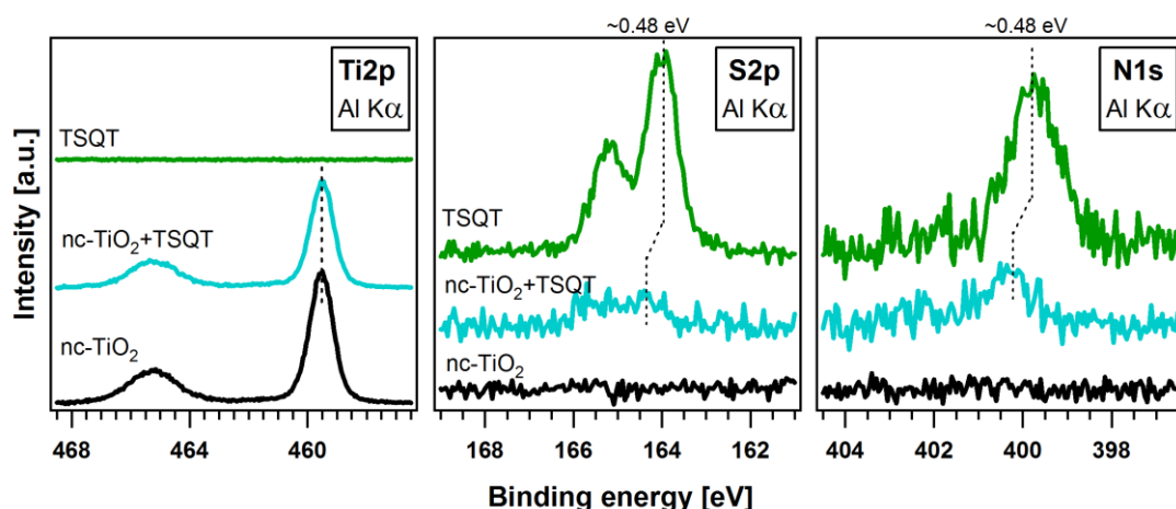
Figure 9.9: Photoemissions from Ti2p, S2p and N1s core levels. The binding energy position of the Ti2p emission does not change in the composite. A difference of \sim 0.48 eV is found for the binding energies of the S2p and N1s emissions of the composite from that of the pristine TSQT.
