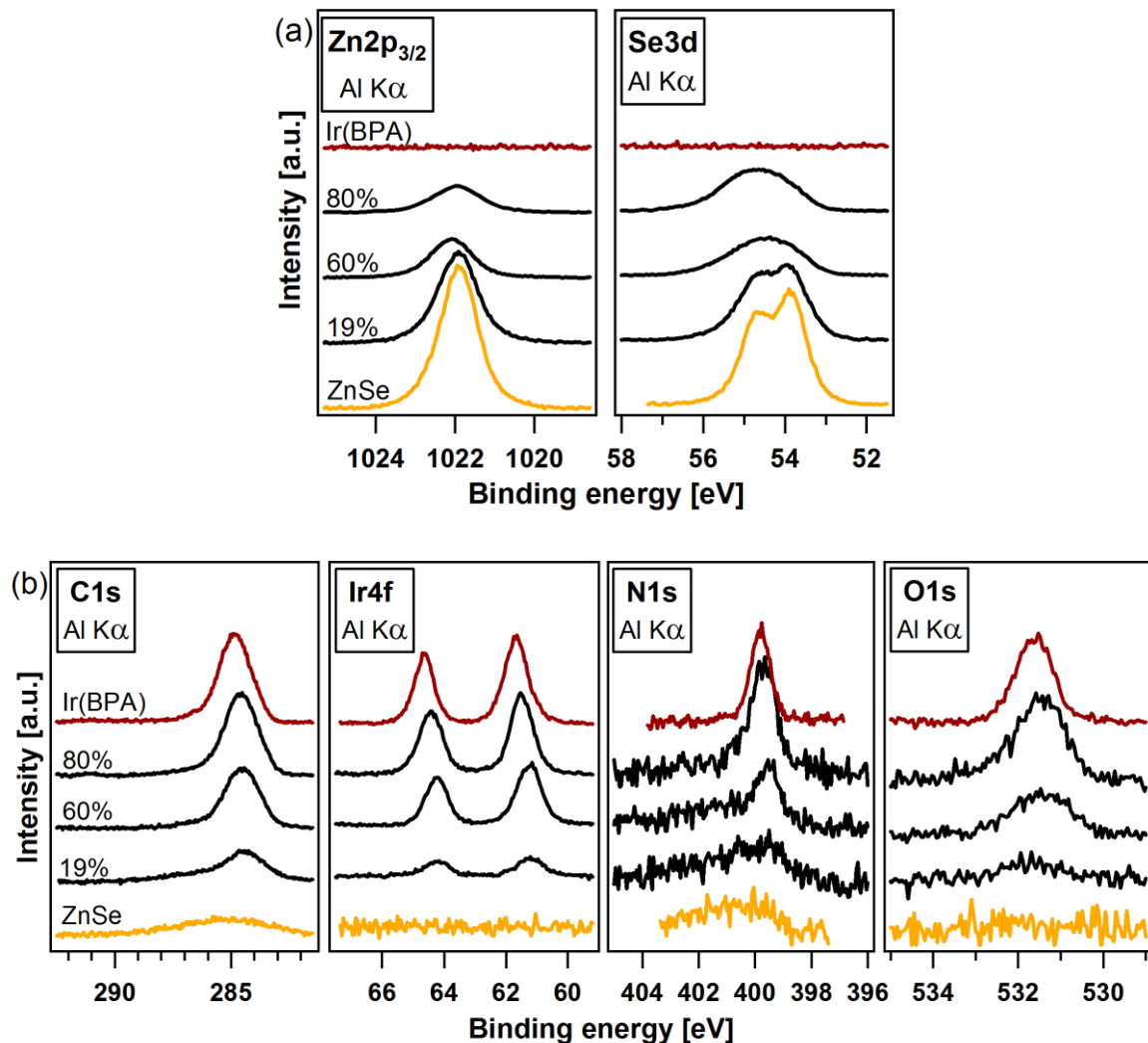
Figure 5.16: Zn 2p_{3/2} and Se 3d core level emission spectra (a), C 1s , Ir 4f , O 1s and N 1s core level emission spectra of Ir(BPA) (b). The dye volume percentages are indicated. The spectra of pristine ZnSe and Ir(BPA) are added. The Se 3d spectra show a gradual broadening with increased dye concentration.
