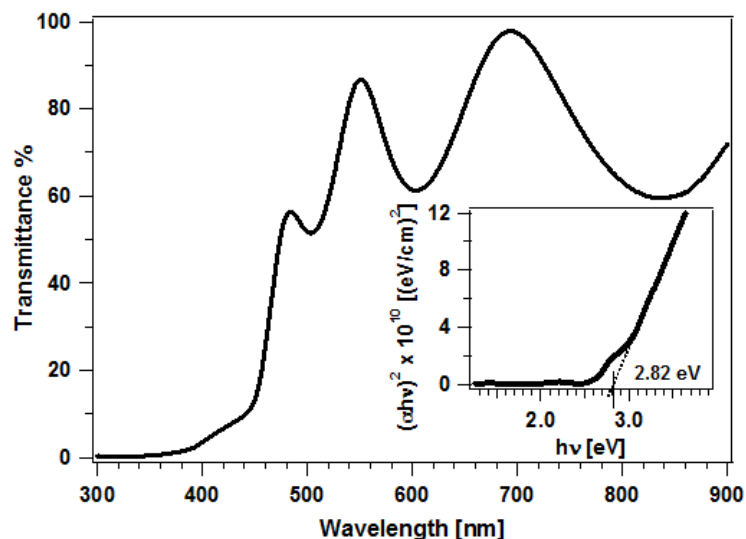
Figure 4.10: Optical transmission of the 440 nm ZnSe film deposited from a freshly-filled source. The inset shows the two direct transitions of ZnSe. The 2.82 eV is the ZnSe energy gap for the allowed direct transition.
