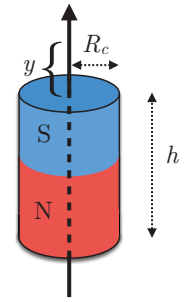
Figure 1.13: Representation of the magnet.
