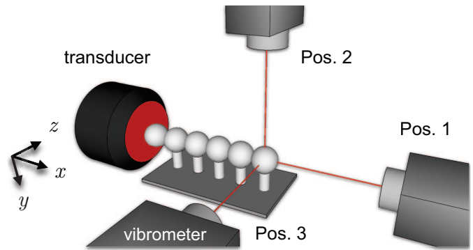
Figure 2.8: Schematics of the experimental setup. The configuration allows us to drive the chain along x , y or z directions. We place the vibrometer in 3 different positions, Pos. 1, 2 and 3 to detect displacement along the x , y and z axis, respectively.
