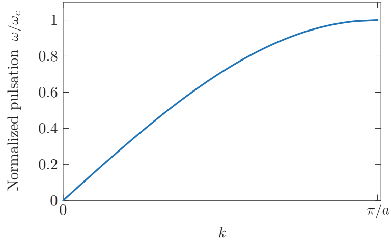
Figure 1.9: Dispersion relation for the longitudinal mode in one-dimensional granular chain.
