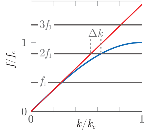
Figure 3.13: Representation of the dispersion curve of a monoatomic granular chain, linear relation and representation of the wave number mismatch \Delta k .
