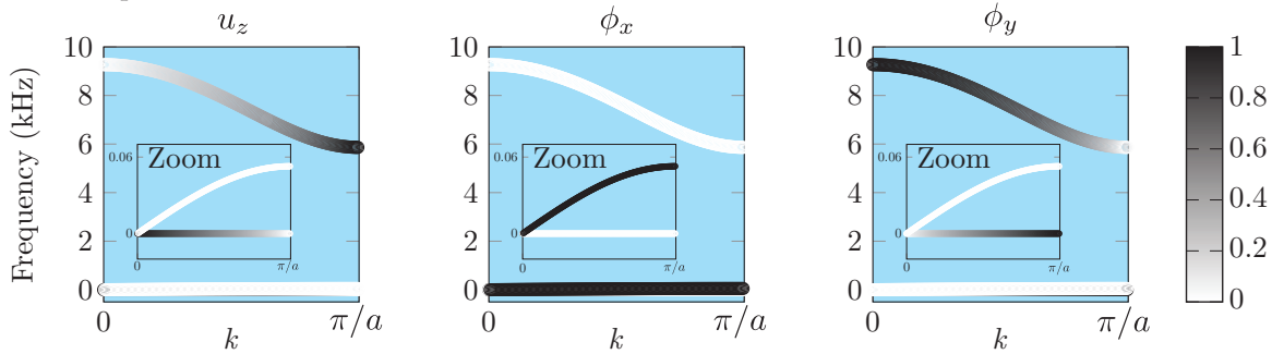
Figure 2.5: Relative amplitude of the components for each mode polarized in (a) sagittal and (b) horizontal planes for the free granular chain. Colors white and black correspond to absence (0) and pure existence (1) of the component, respectively.
