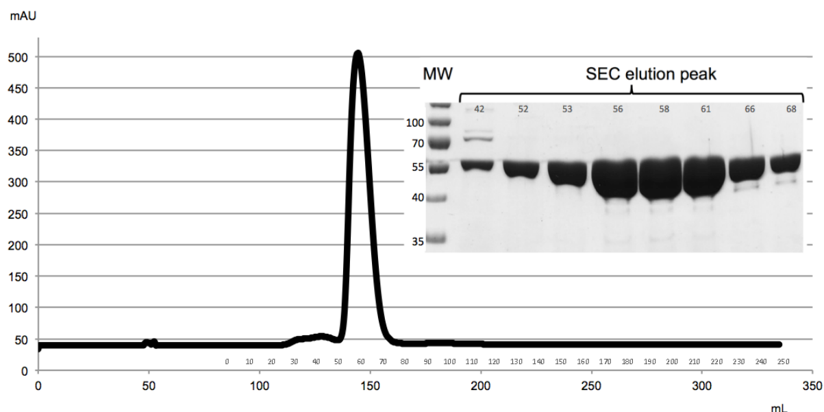
Fig. 40 Chromatogram of His-EngA WT purification using a Superdex® 75 column for size exclusion chromatography. Elution is followed by measurement of UV absorbance at 280 nm collected over the elution volume. Small numbers on the x-axis represent fractions collected during elution. The inset represents the SDS-PAGE analysis of the elution peak with the labelled fractions analysed. (MW) molecular weight marker.
