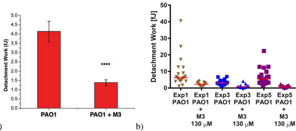
Figure 5.6: a) Data distribution of W_D obtained for 16HBE vs. PAO1 wild-type with and without M3. Median \pm SEM are presented. p -values: **** p < 0.0001 . b) Detachment work with and without M3. Data from three different experiments are presented. Median is represented as red bar.
