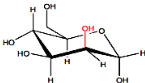
Figure 1.8: D-Mannose structure.
