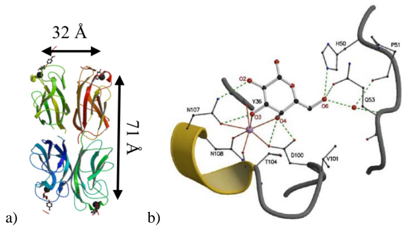
Figure 1.2: a) Crystal structure of LecA complex with GalA-QRS at 2.31 Å resolution (4LKD) [55]; dimensions are 32 X 71 X 19 Å. b) View of the calcium and galactose binding site in the crystal structure from [15].
