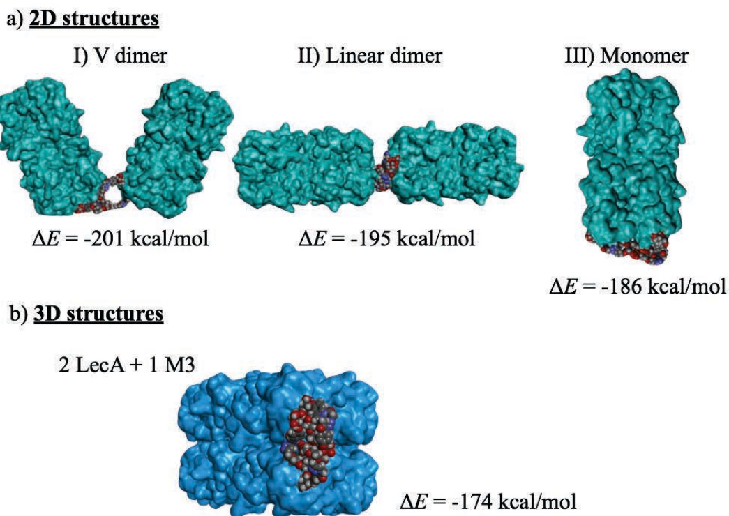
Figure 3.13: MD simulations of a) 2D and b) 3D arrangement of the most energetically favorable interactions between M3 glycocluster(s) and LecA lectin(s) monomers.
