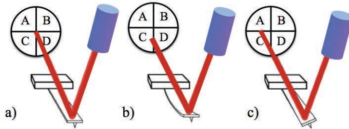
Figure 2.7: Laser beam detection of the cantilever deflection.
