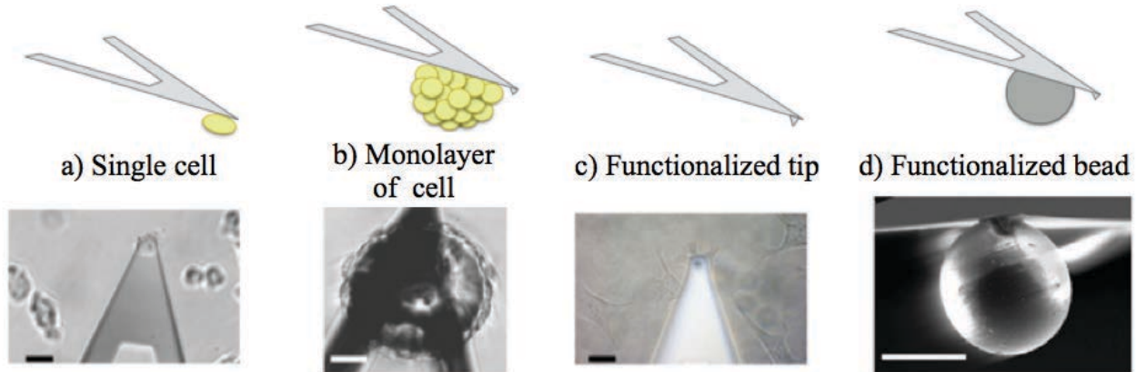
Figure 2.25: Sketches and microscopy images of the different functionalization techniques used in SCFS studies. Adapted from [149].
