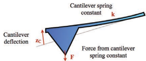
Figure 2.11: Relation between the tip-sample interaction force F and the cantilever deflection z_c and the spring constant k .
