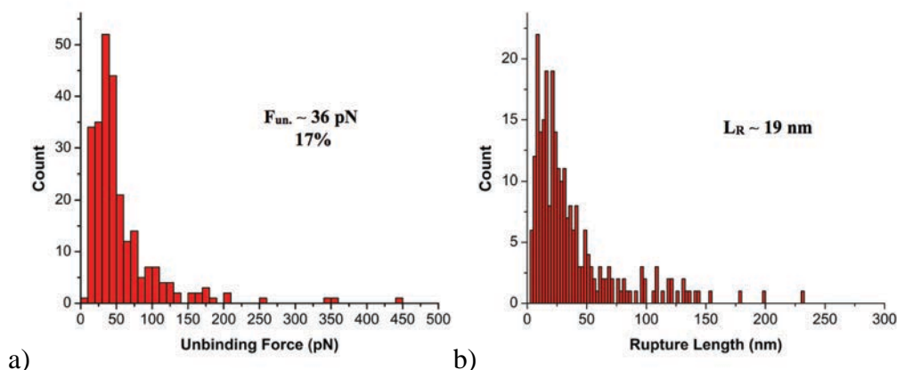
Figure 4.16: Data distribution of a) unbinding force and b) rupture length for the interaction with D1 glycocluster at pulling speeds v = 100 nm/s.
