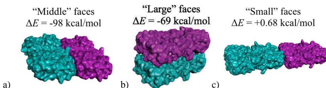
Figure 3.7: MD simulation of lectin/lectin interaction along a) lectin’s “middle” faces, with a potential energy of \Delta E = -98 kcal/mol; b) lectin’s “large” faces, with a potential energy of \Delta E = -69 kcal/mol; c) lectin’s “small” faces, with a potential energy of \Delta E = +0.68 kcal/mol, not an energetically favorable interaction.
