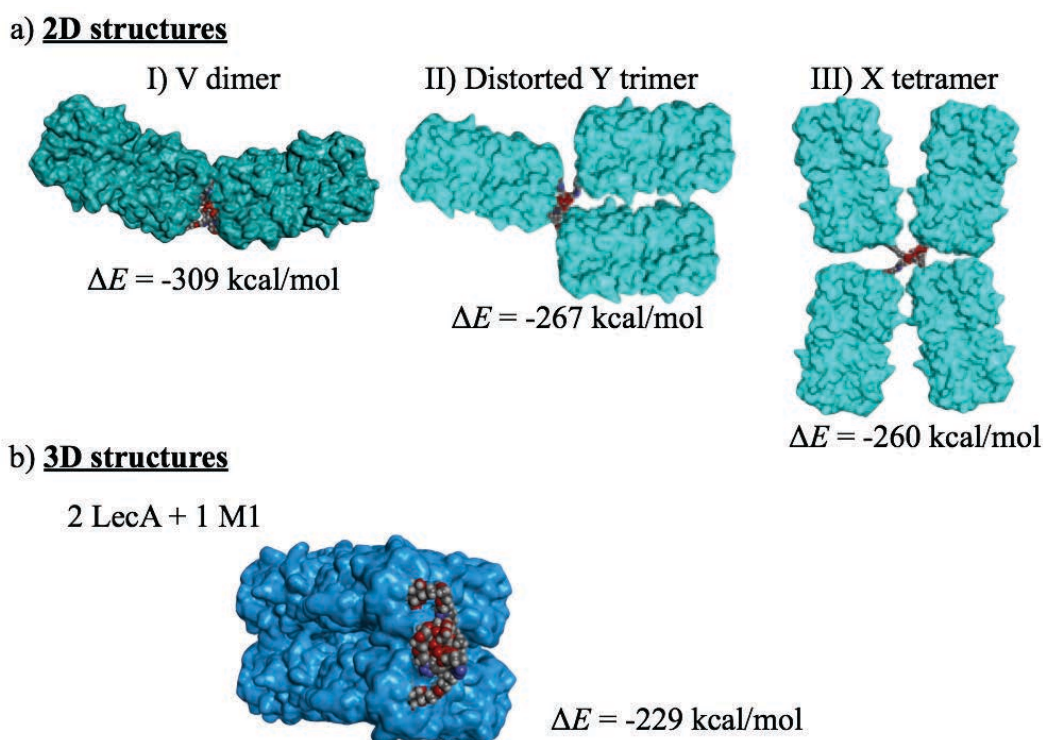
Figure 3.9: MD simulations of a) 2D and b) 3D arrangement of the most energetically favorable interactions between M1 glycocluster(s) and LecA lectin(s) monomers.
