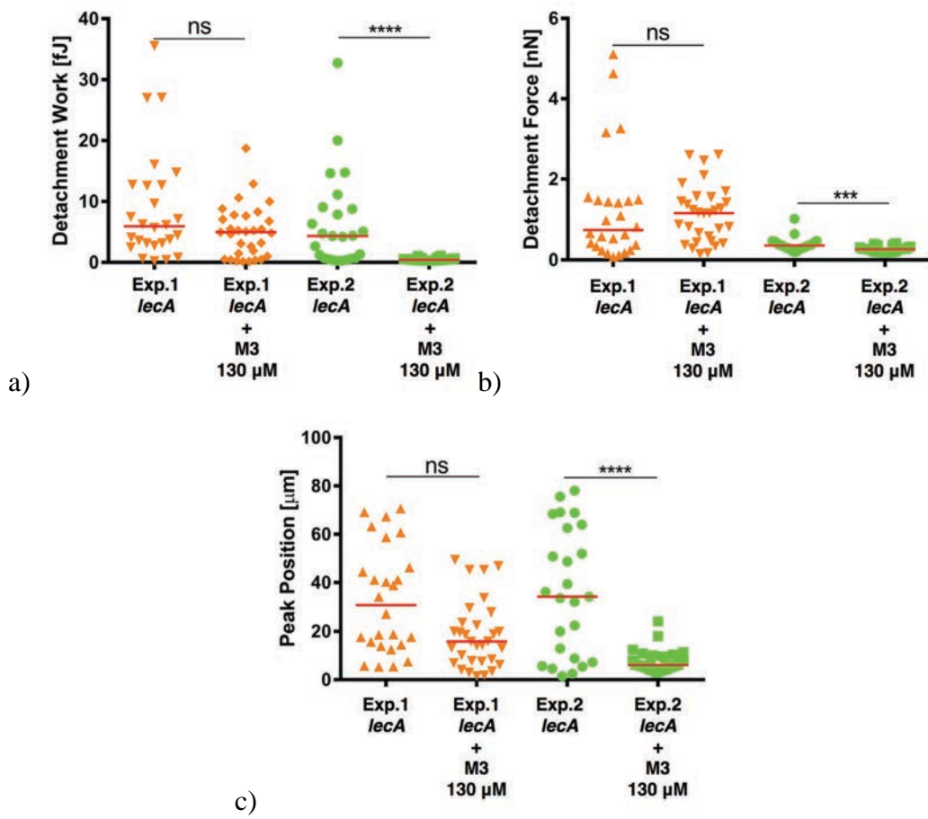
Figure 5.11: a) Detachment work and b) detachment force and c) peak position for 16HBE vs. lecA mutant with and without M3. Data from two different experiments are presented. Median is represented as red bar, p values are: ns not significant difference, *** p < 0.001 and **** p < 0.0001 .
