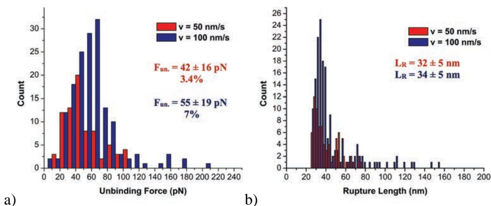
Figure 4.21: Data distribution of a) unbinding force and b) rupture length obtained for M3 glycocluster at pulling speed v = 50 nm/s (red) and v = 100 nm/s (blue).
