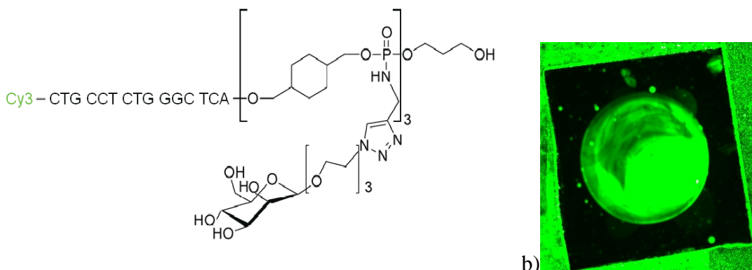
Figure 4.5: a) Complementary DNA sequence bearing the fluorescent tag and the glycocluster D1; b) Fluorescent image of a hybridized sample.
