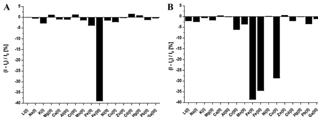
Fig. 2. Change in fluorescence emission of compound 1 (A) and 4 (B) ( 0.5 \mu\text{M} , \lambda_{\text{exc}} = 292 \text{ nm} , water) upon addition of 200 equivalents of various metal cations as perchlorate salts.
