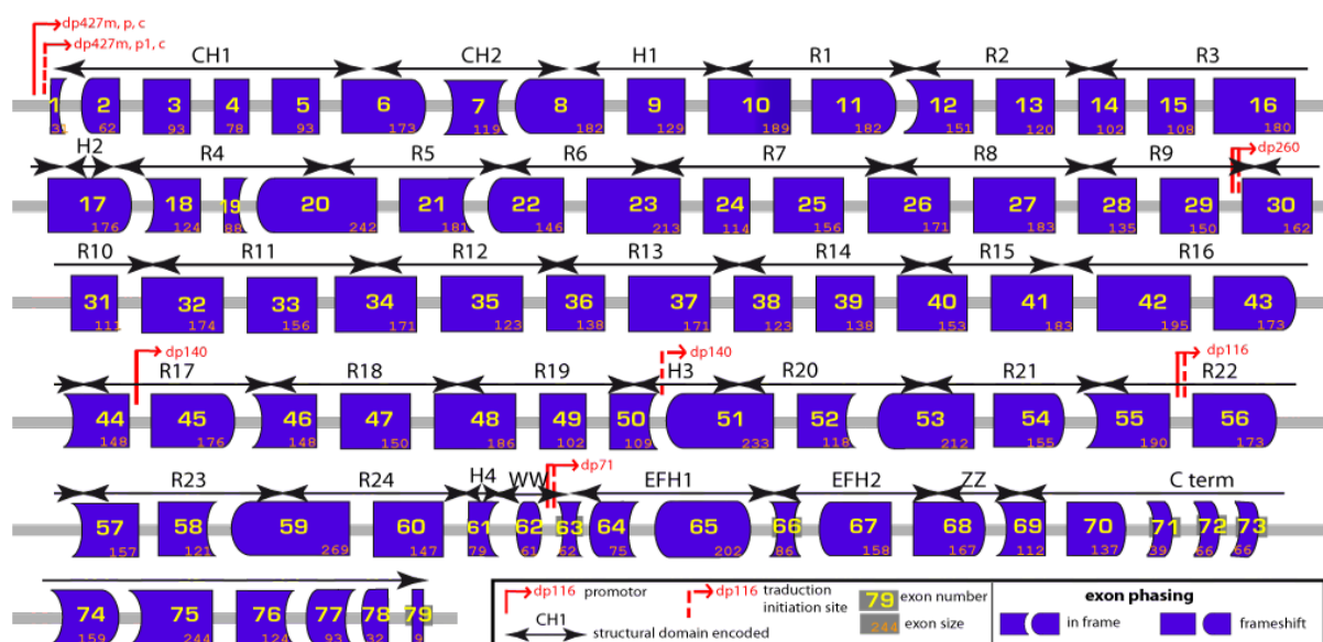
Figure 1. Representation of the domains encoded by the exons within the dystrophin gene. Figure from Nicolas et al. 2012 (Nicolas et al., 2012). Deletions of exons which result in-frame deletions result in a truncated dystrophin to be expressed whereas exon deletions resulting in a frameshift of the reading frame will result in an unstable protein.
