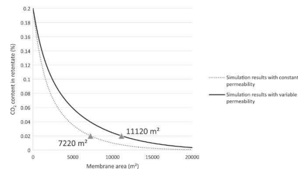
Fig. 10. Retentate composition as a function of membrane module area for a 6FDA TAPDO membrane (thickness 2 \mu m) with a 80/20 CH 4 /CO 2 feed mixture under cross plug flow conditions.
