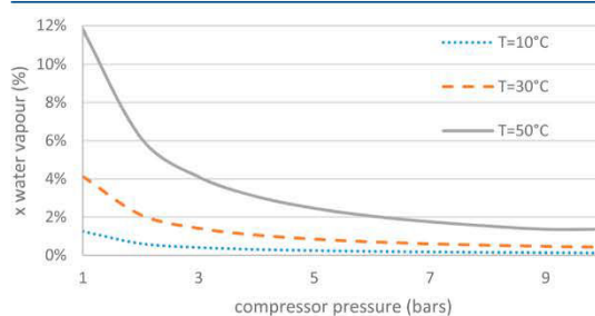
Figure 4. Water vapor volume fraction from a compressor/heat exchanger cooler outlet stream. A saturated flue gas is taken at the temperature indicated on the curves for inlet compressor conditions. The inlet saturated feed flow composition in dry basis is 13.3% CO 2 , 81.1% N 2 , and 5.6% O 2 .
