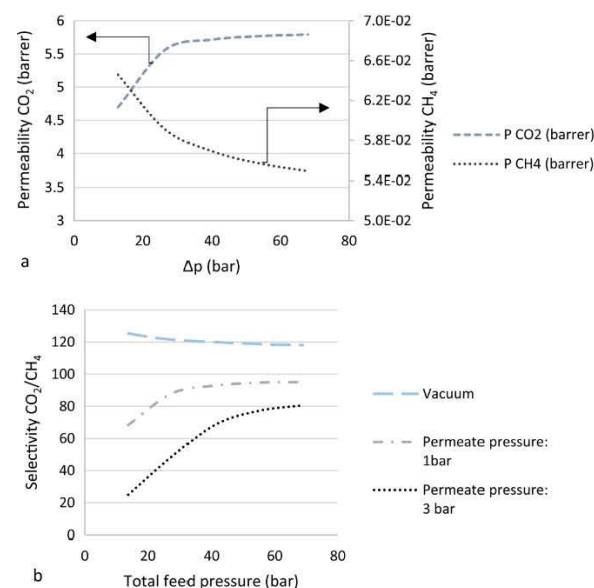
Fig. 8. Simulation of the influence of different upstream / downstream pressure conditions on effective CO 2 /CH 4 selectivity. Same conditions as Fig. 7, except pressure.
