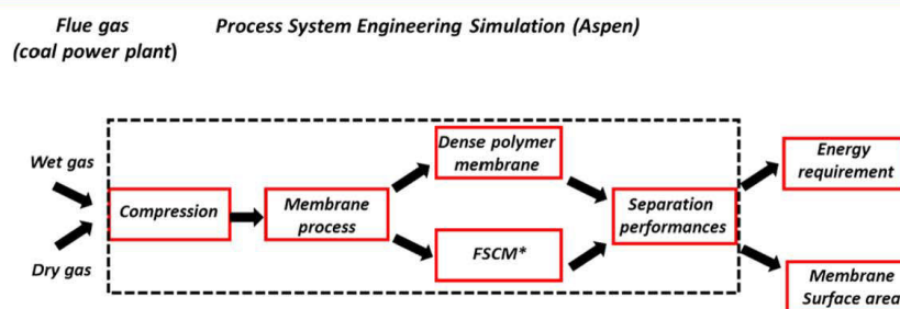
Figure 2. Overall framework of the study: A wet or dry flue gas mixture is compressed and separated in a single-stage membrane unit. For each set of operating conditions, the separation performances of the membrane unit (carbon dioxide purity, y , and recovery, R ) are computed through PSE (Aspen software) and the corresponding specific energy requirement ( E ) and membrane surface area ( A ) are calculated. [*Fixed site carrier membrane (chemically reactive membrane).]
