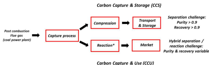
Figure 1. CCS versus CCU overall framework. [*CO 2 transformation processes include chemical (thermochemical, catalytic), biochemical (fermentation, algae), electrochemical, and mineralization.]
