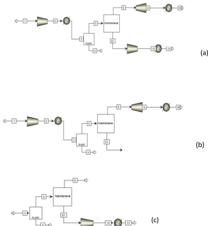
Figure 5. Driving force strategies: (a) compression and vacuum, (b) compression, and (c) vacuum.
