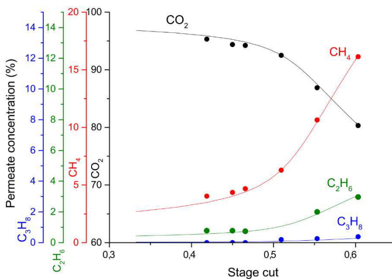
Fig. 14. Permeate concentration as a function of stage cut for one stage permeation. Model results are represented by solid lines and compared to experimental from Pan (symbols) [58].
