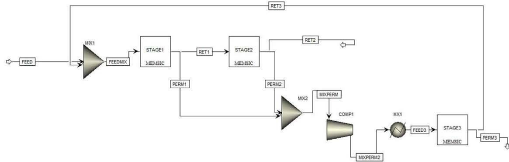
Fig. 13. Multistage membrane separation process for the recovery of CH 4 and CO 2 enriched streams.
