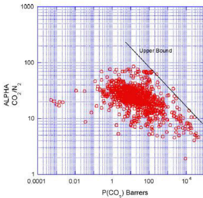
Upper bound correlation for CO 2 /N 2 separation.
