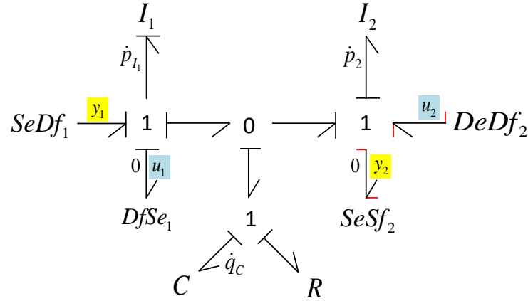
FIGURE 4.32 – Modèle bond graph inverse du bond graph bicausal de la figure 4.26
