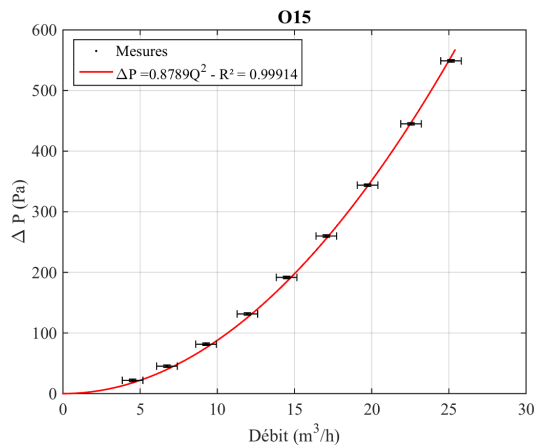
FIGURE C.23 – Extraction du local D
