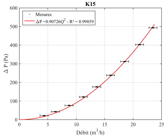
FIGURE C.19 – Soufflage du local D
