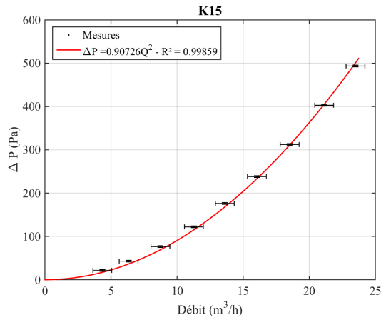
FIGURE C.19 – Soufflage du local D
