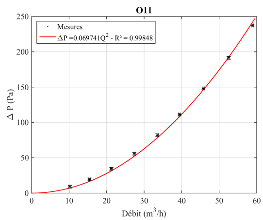
FIGURE C.22 – Extraction du local C
