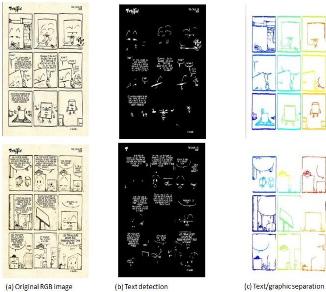
Figure 25: Text/graphic separation in the case of black text written in a non-white speech balloon. (a) RGB processed comics. (b) Text detection results. Some false positives are highlighted. (c) Final results of text extraction from graphics. Graphical components are restored.
