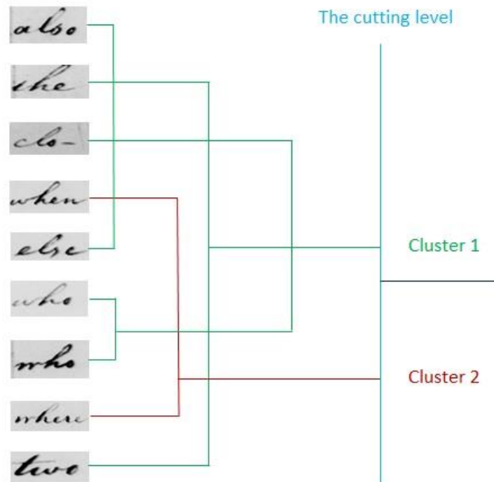
Figure 81: The HAC process for a given query "also".
