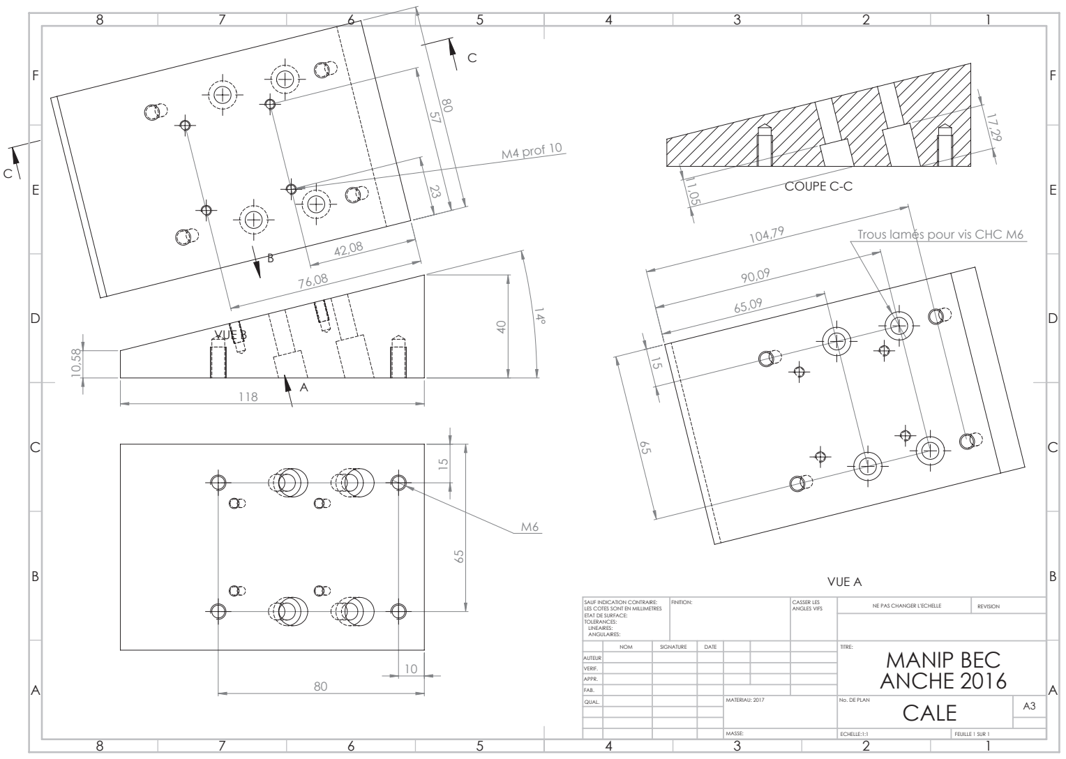
FIGURE D.12: Dimensioned drawing of the angled support (16). Provided by LAUM mechanical workshop.
