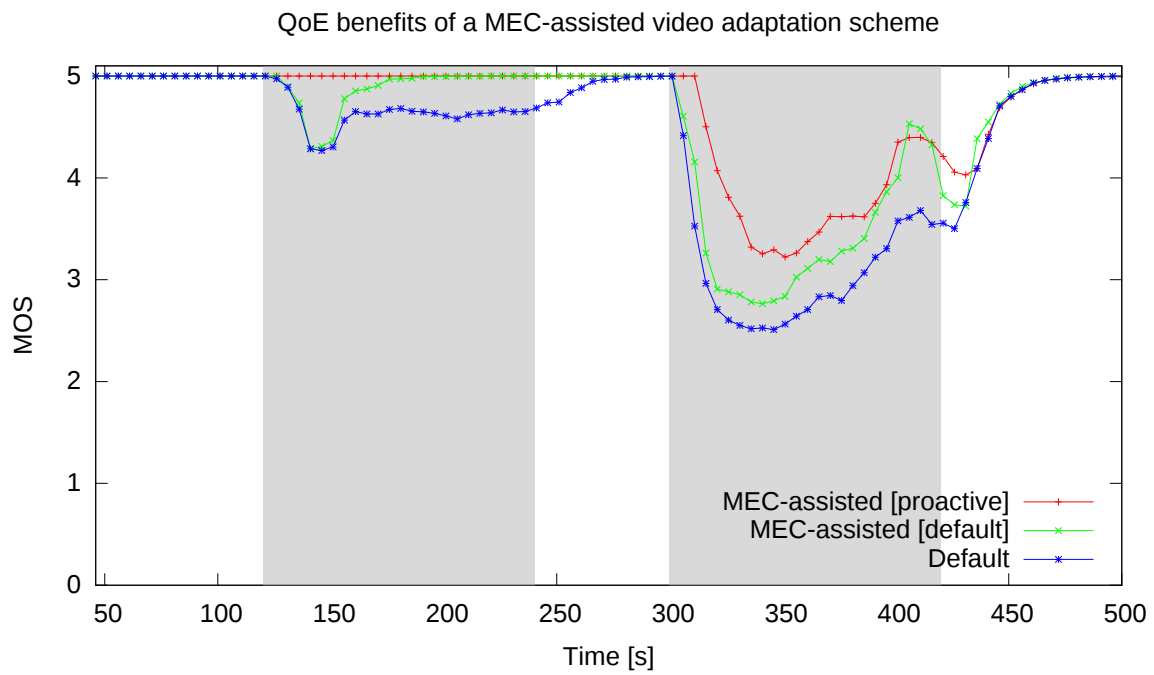
Figure 5.6 – MOS across all 10 Users.
