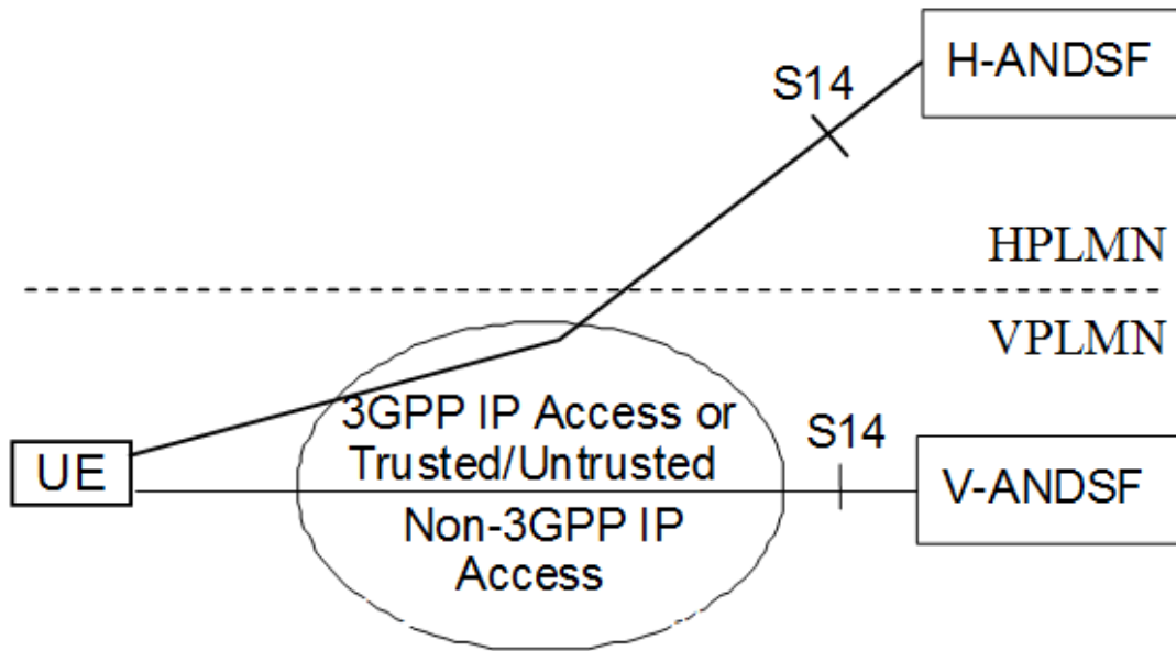
Figure 2.6 – ANDSF architecture
