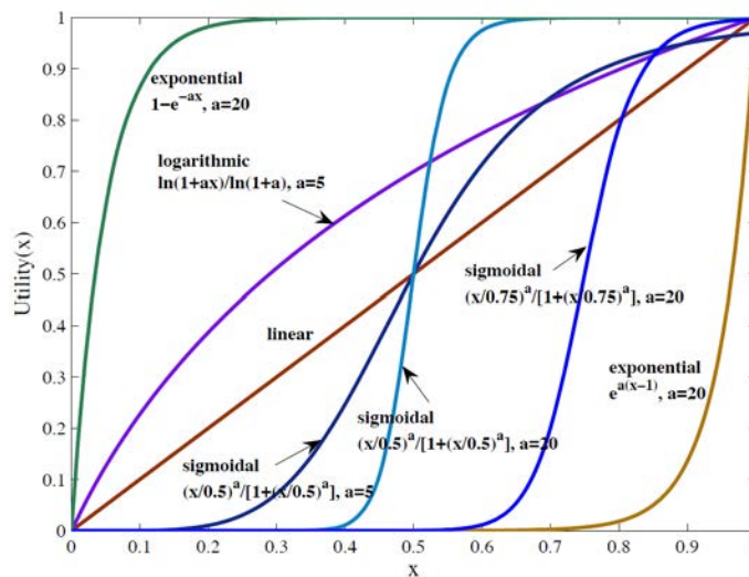
Figure 2.3 – Sigmoid Function Examples, source [16].
