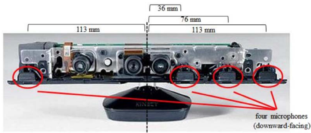
Figure 3.3: Linear array of 4 microphones inside the Kinect sensor ( https://www.microsoft.com ).
